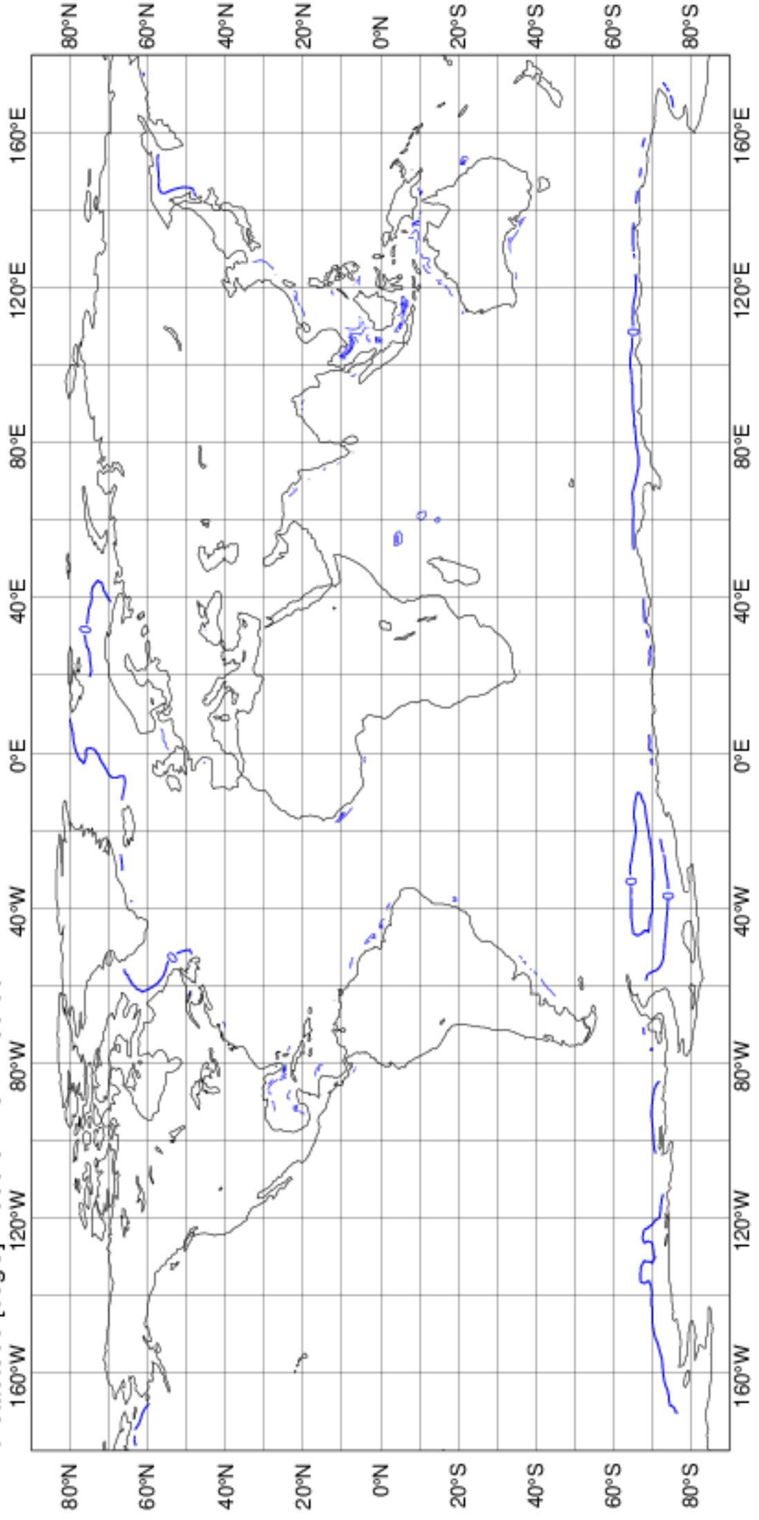
thetao300 [degC] 2000-01-16T12:00:00
