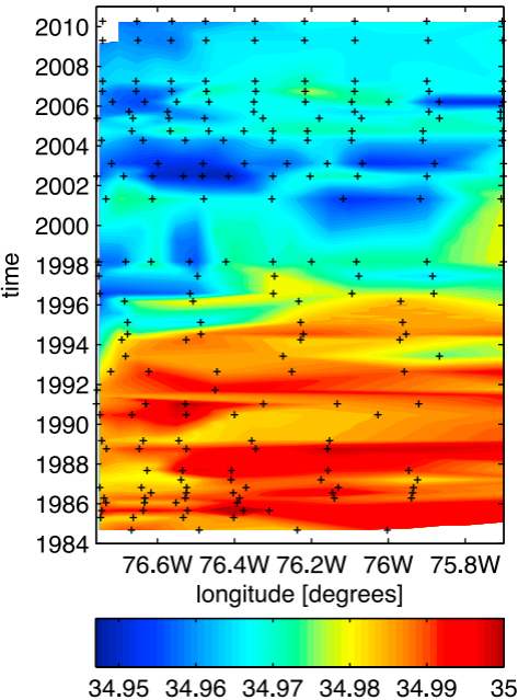
(a) Salinity at \sigma_{1.5} = 34.67
