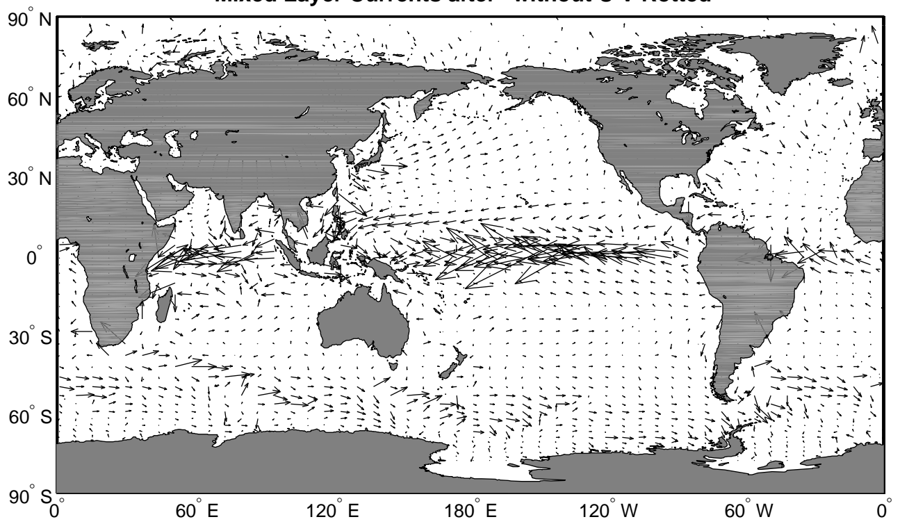
Mixed Layer Currents after "without U V Rotted"
