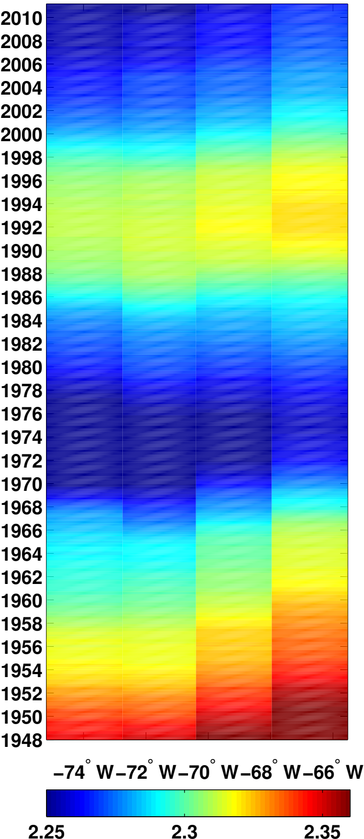
(b) Temperature ( ^{\circ} C) at \sigma_2=36.946
