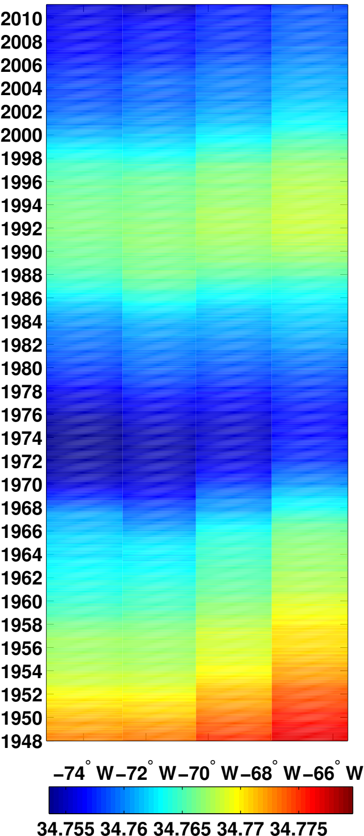
(a) Salinity (psu) at \sigma_2=36.946
