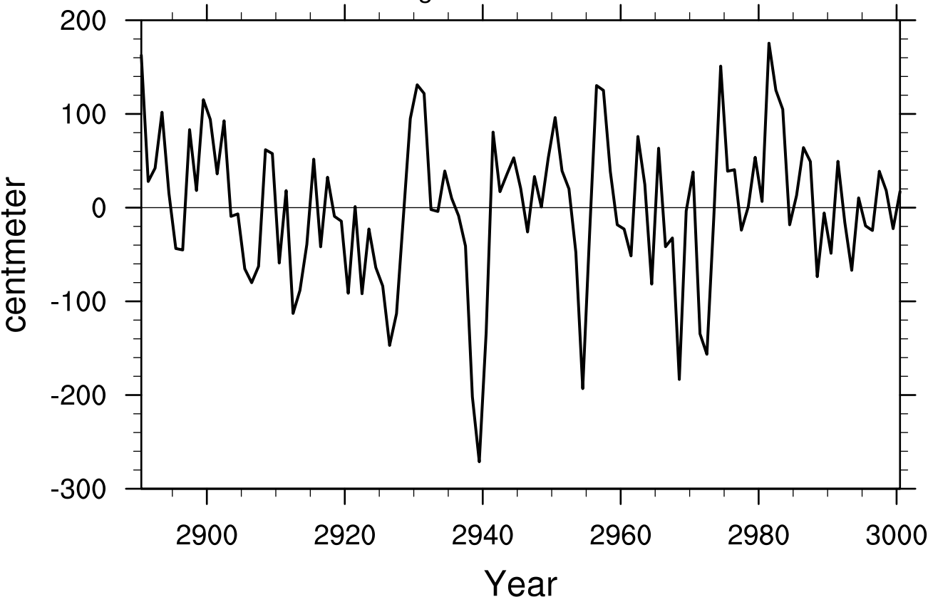
PC3 of Sea Surface Height
