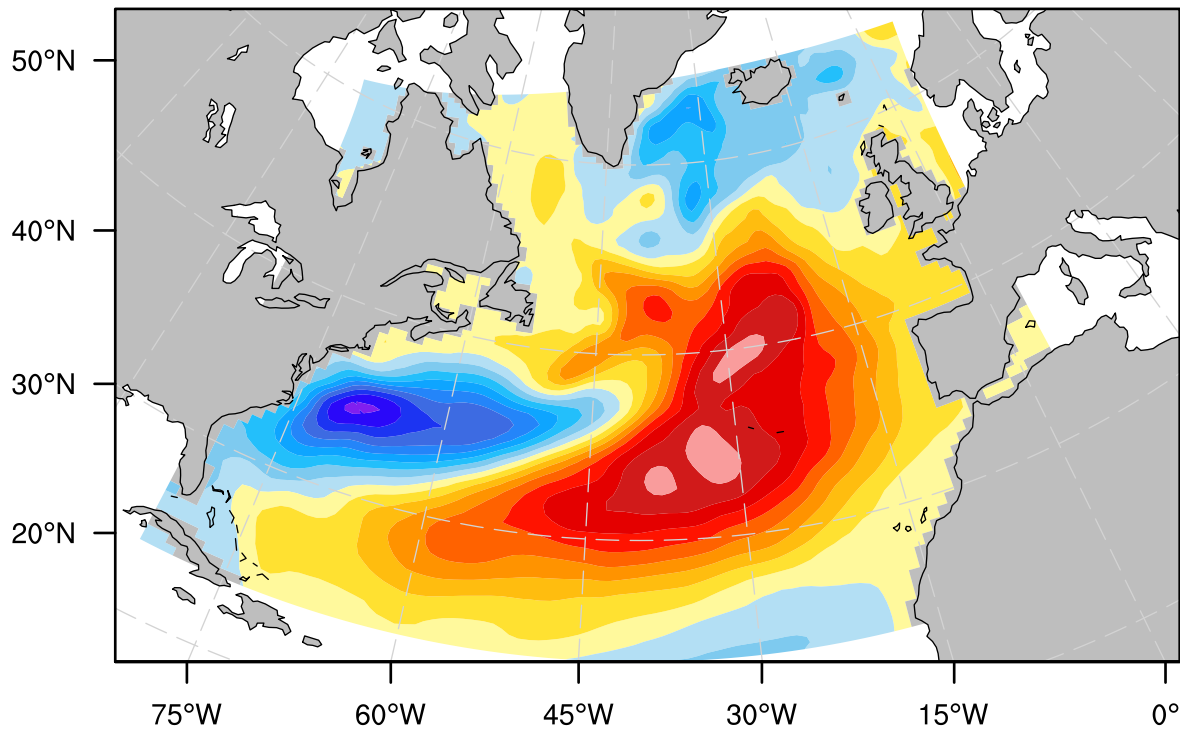
EOF3 of Sea Level Height
