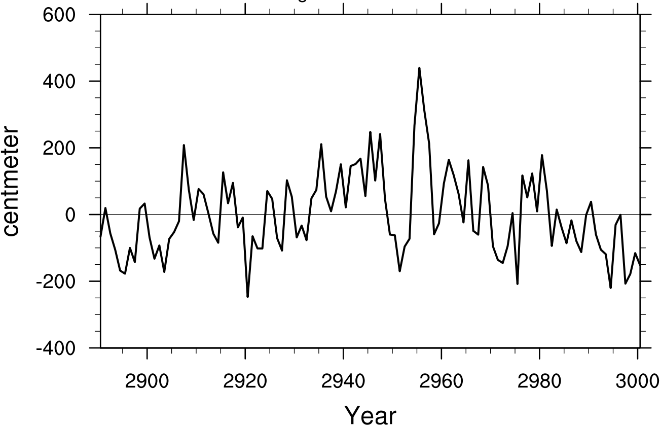
PC1 of Sea Surface Height
