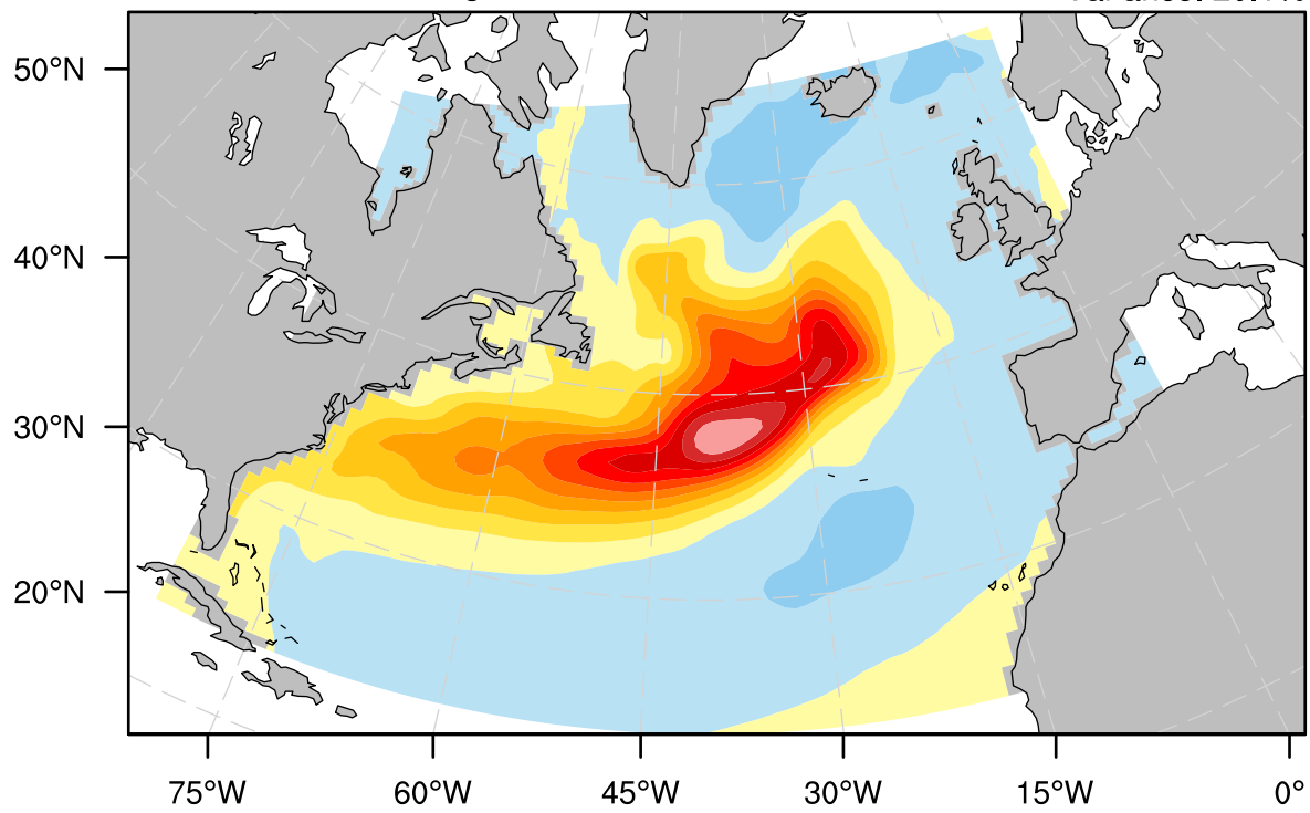
EOF1 of Sea Level Height
