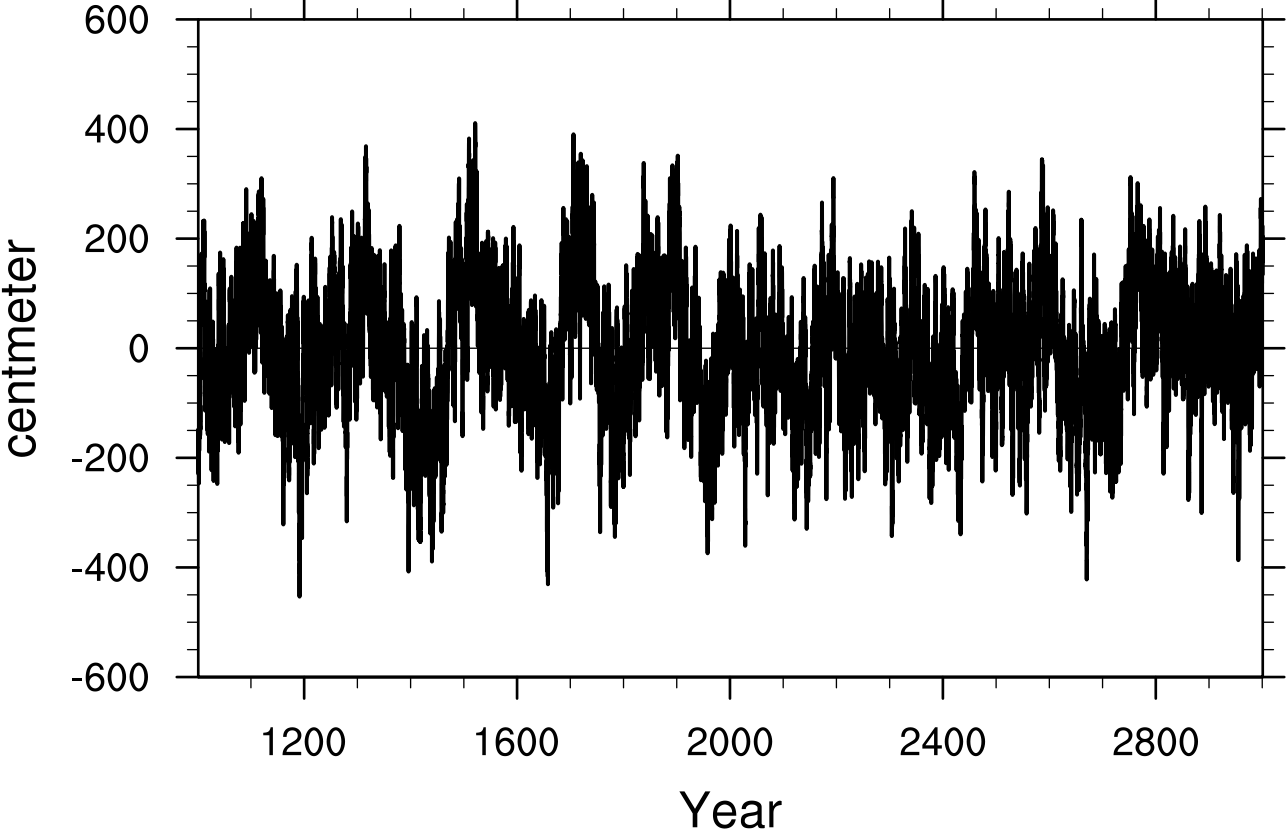
PC1 of Sea Surface Height
