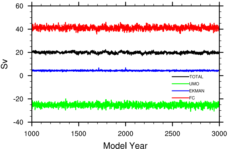
Model simulated AMOC
