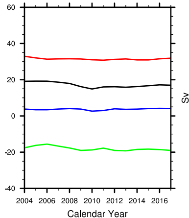
Observed RAPID AMOC
