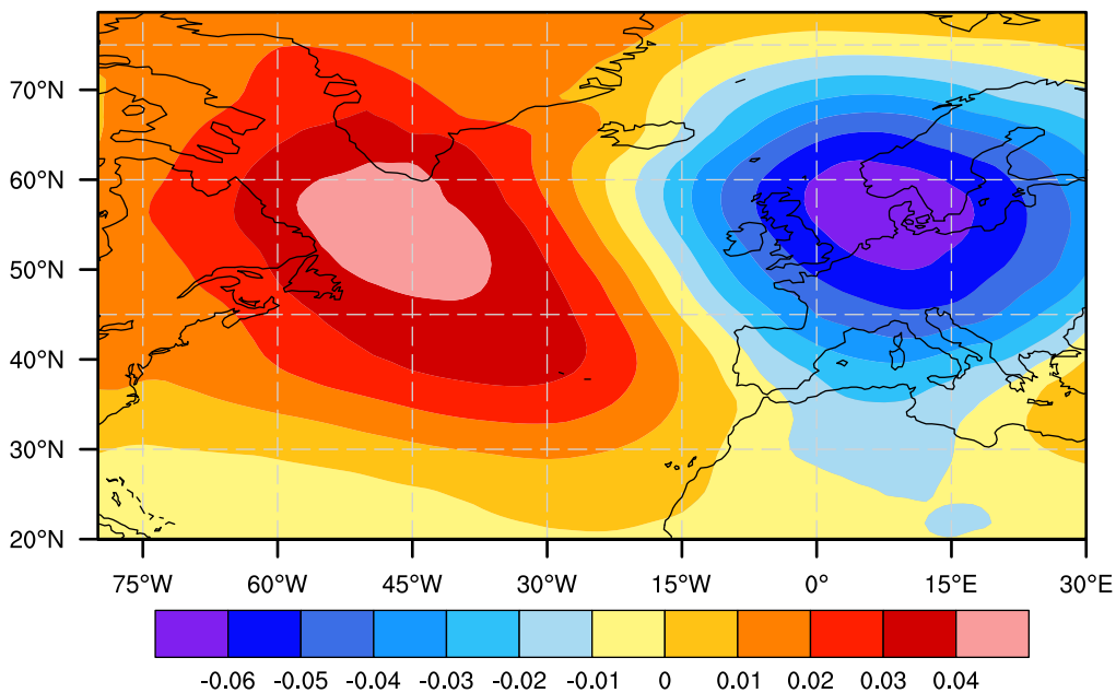
EOF3 of EOF of DJF: Sea level pressure
