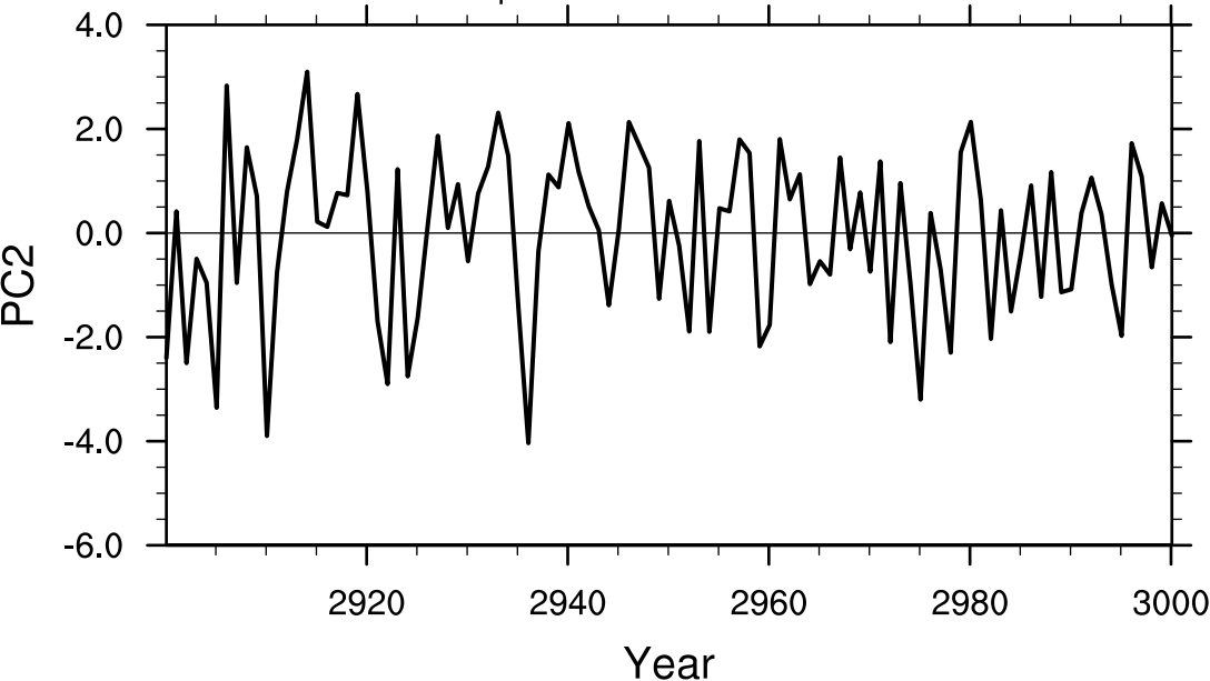
EOF of DJF: Sea level pressure
