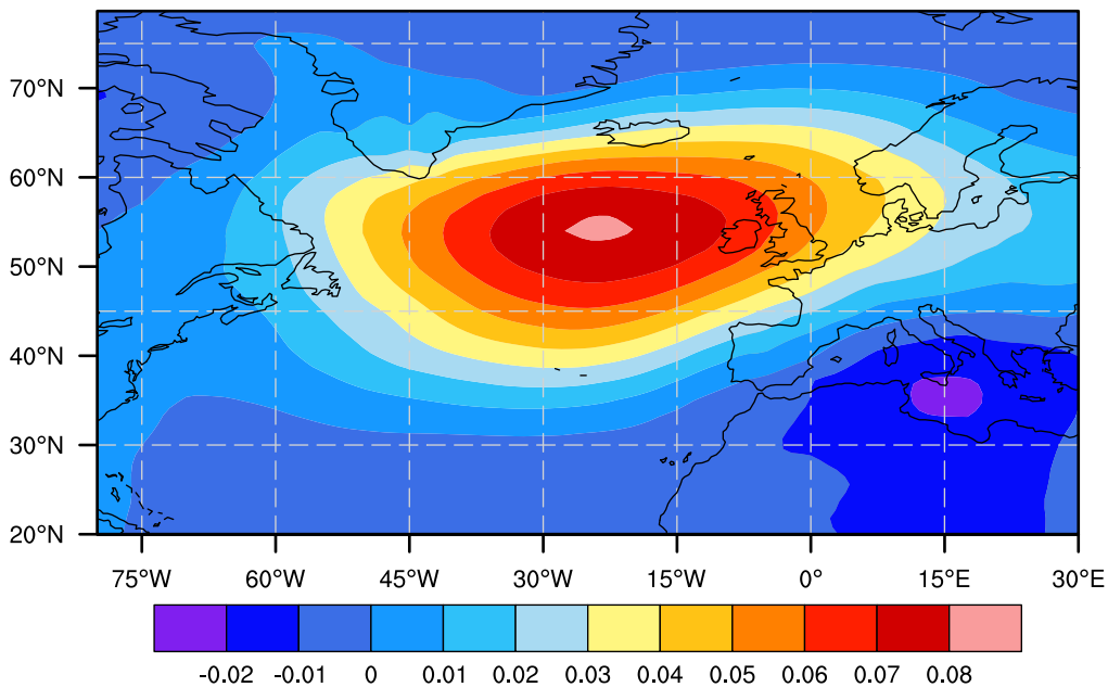
EOF2 of EOF of DJF: Sea level pressure
