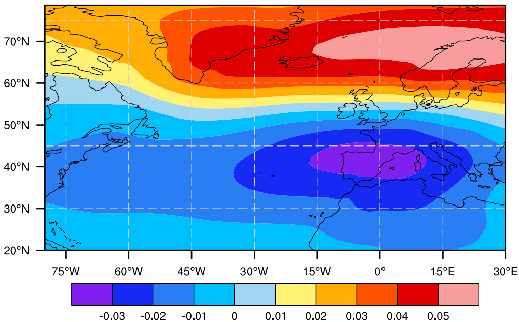
EOF1 of EOF of DJF: Sea level pressure
