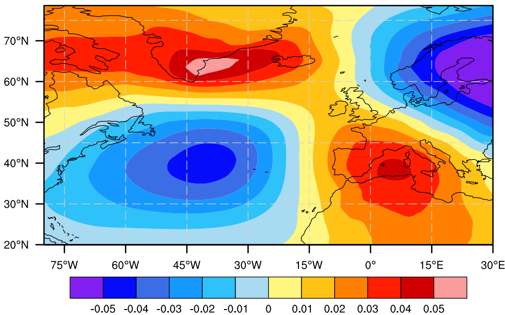
EOF3 of EOF of DJF: Sea level pressure
