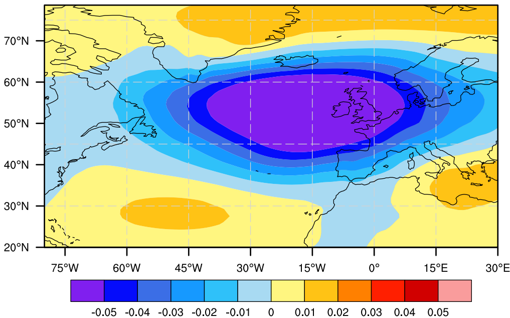
EOF2 of EOF of DJF: Sea level pressure
