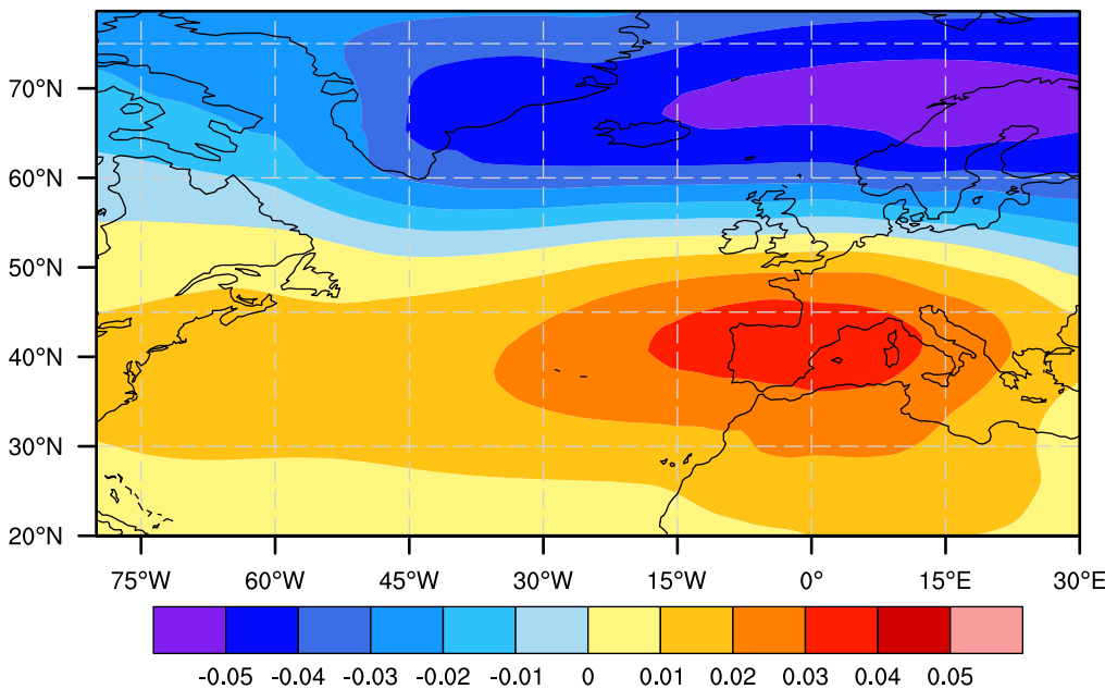
EOF1 of EOF of DJF: Sea level pressure
