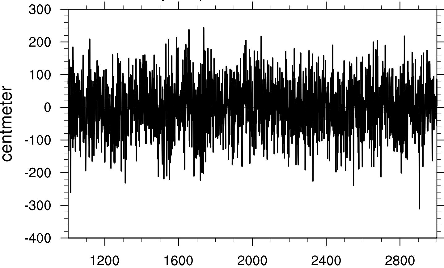
PC3 of Mixed Layer Depth
