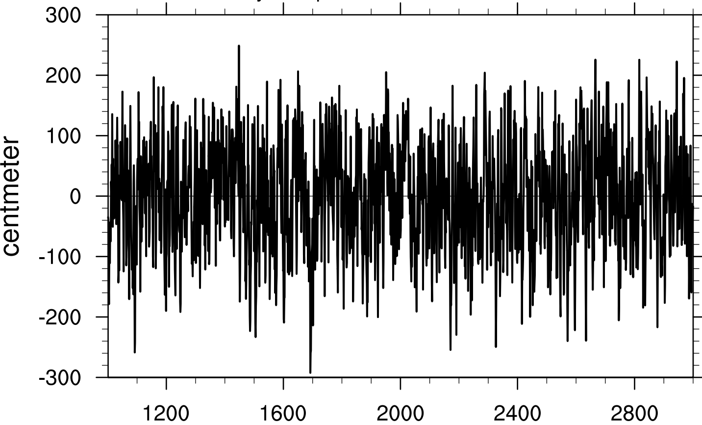
PC2 of Mixed Layer Depth
