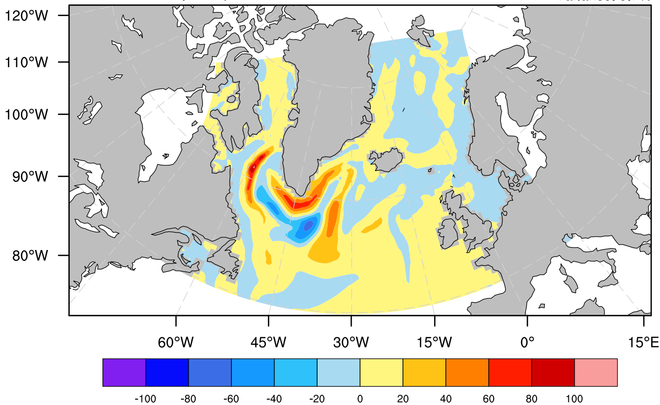
PC2 of Mixed Layer Depth
