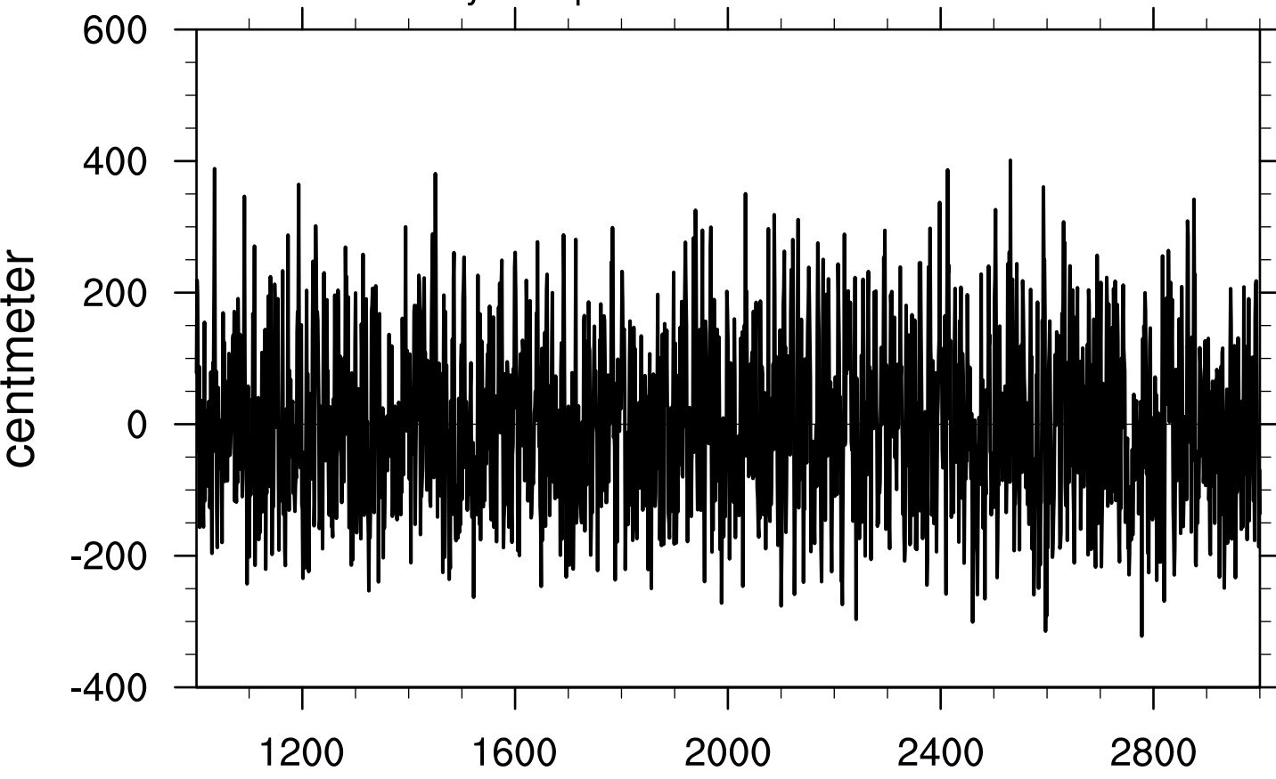
PC1 of Mixed Layer Depth
