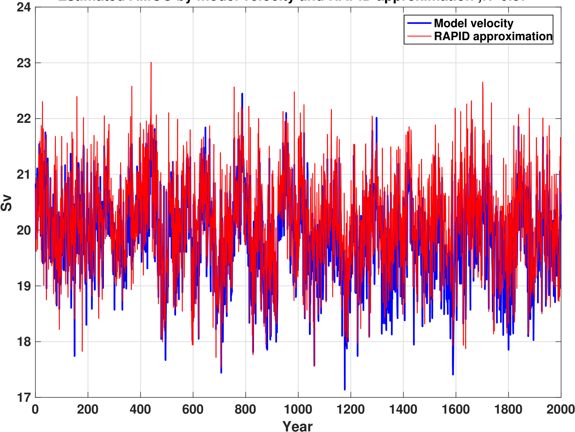
Estimated AMOC by model velocity and RAPID approximation ,R=0.87
