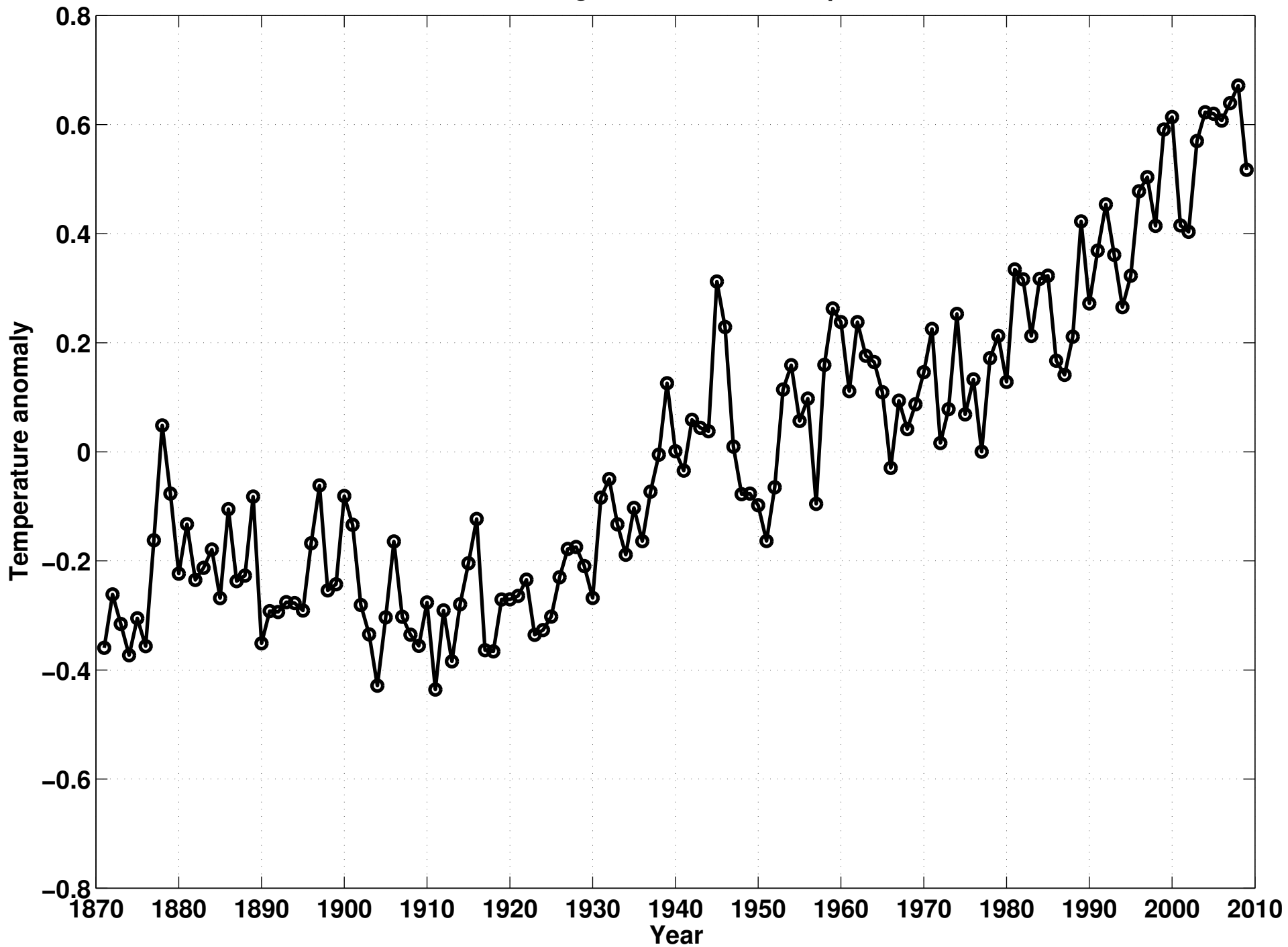
Global averaged surface air temperature
