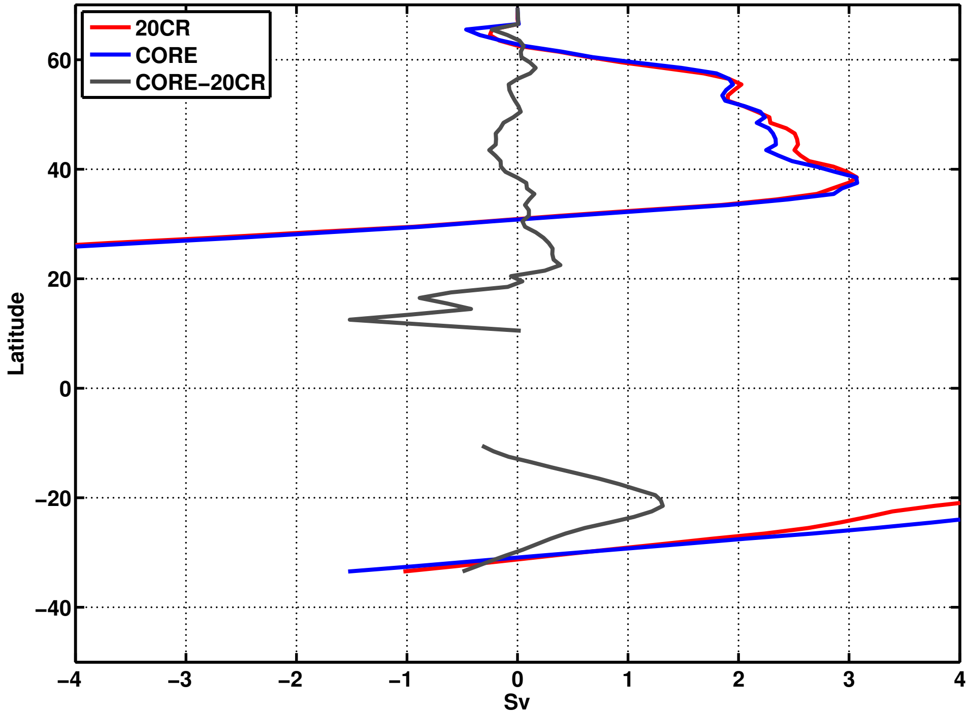
Meridional Ekman transport (positive southward) in the North Atlantic
