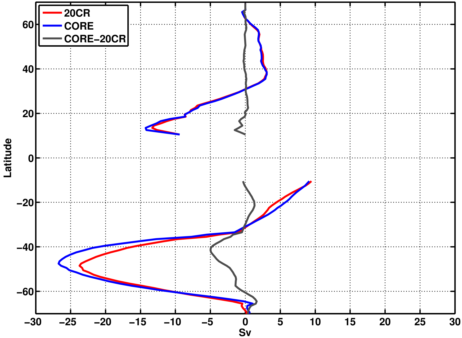
Meridional Ekman transport (positive southward) in the North Atlantic and Southern Ocean
