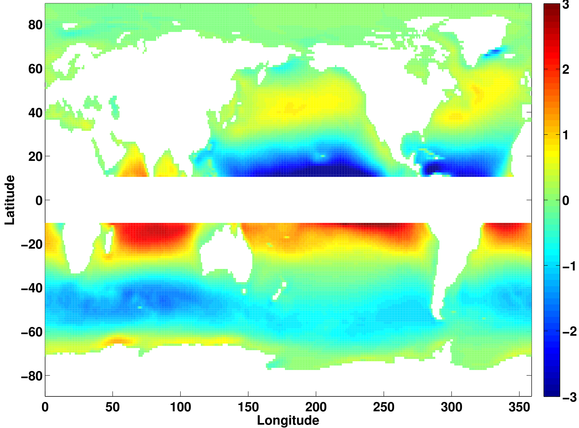
Ekman transport of CORE (unit: \text{m}^3/\text{s}/\text{m} )
