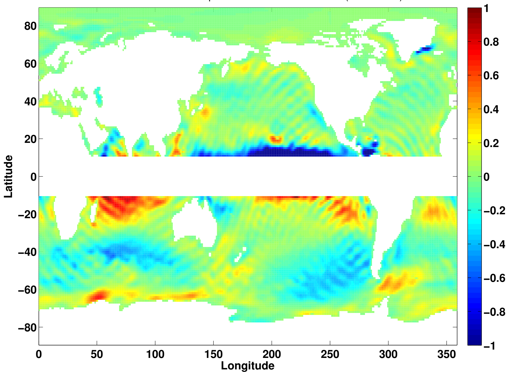
Difference of Ekman transport between 20CR and CORE (unit: \text{m}^3/\text{s}/\text{m} )
