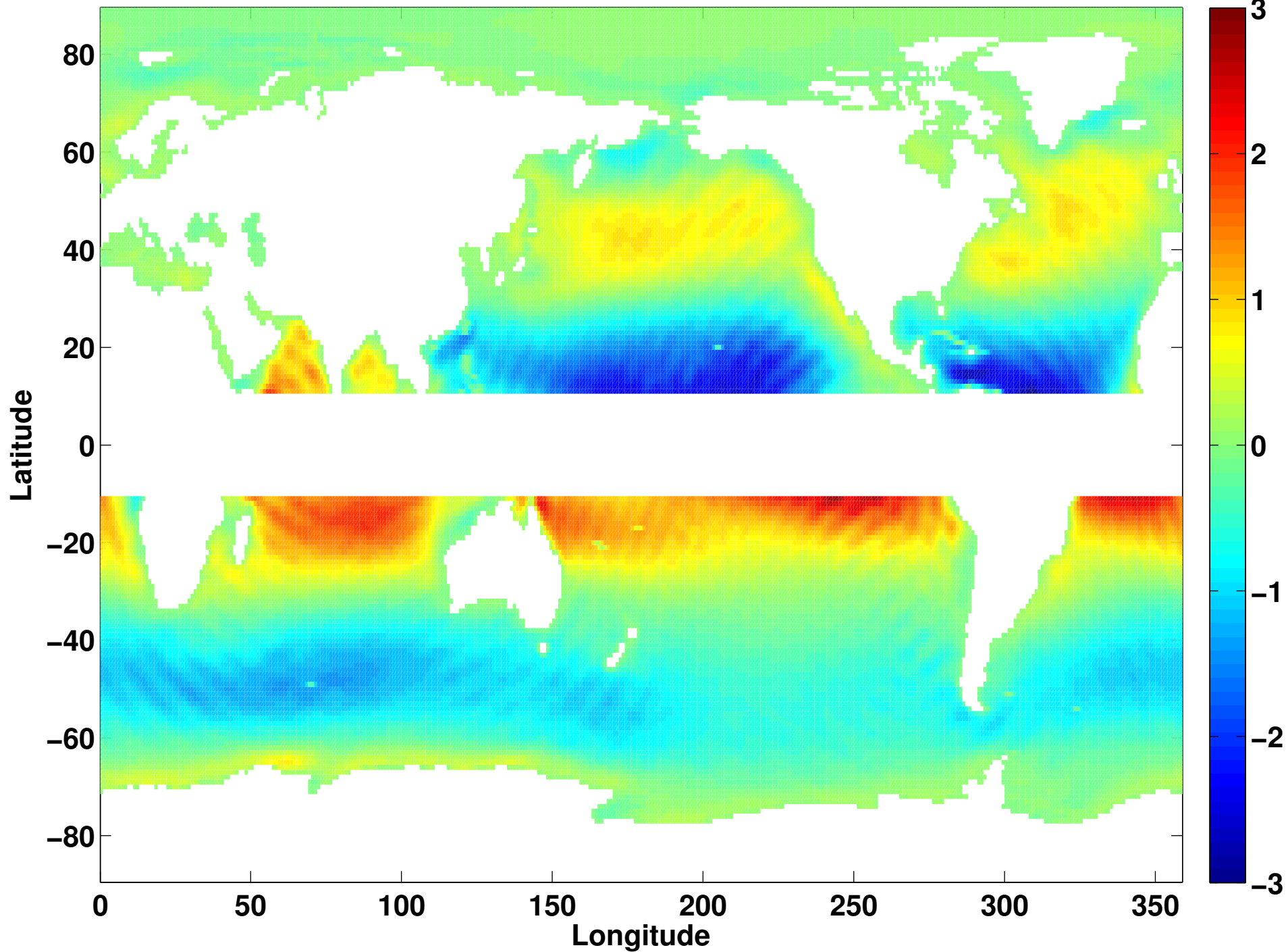
Ekman transport of 20CR (unit: \text{m}^3/\text{s}/\text{m} )
