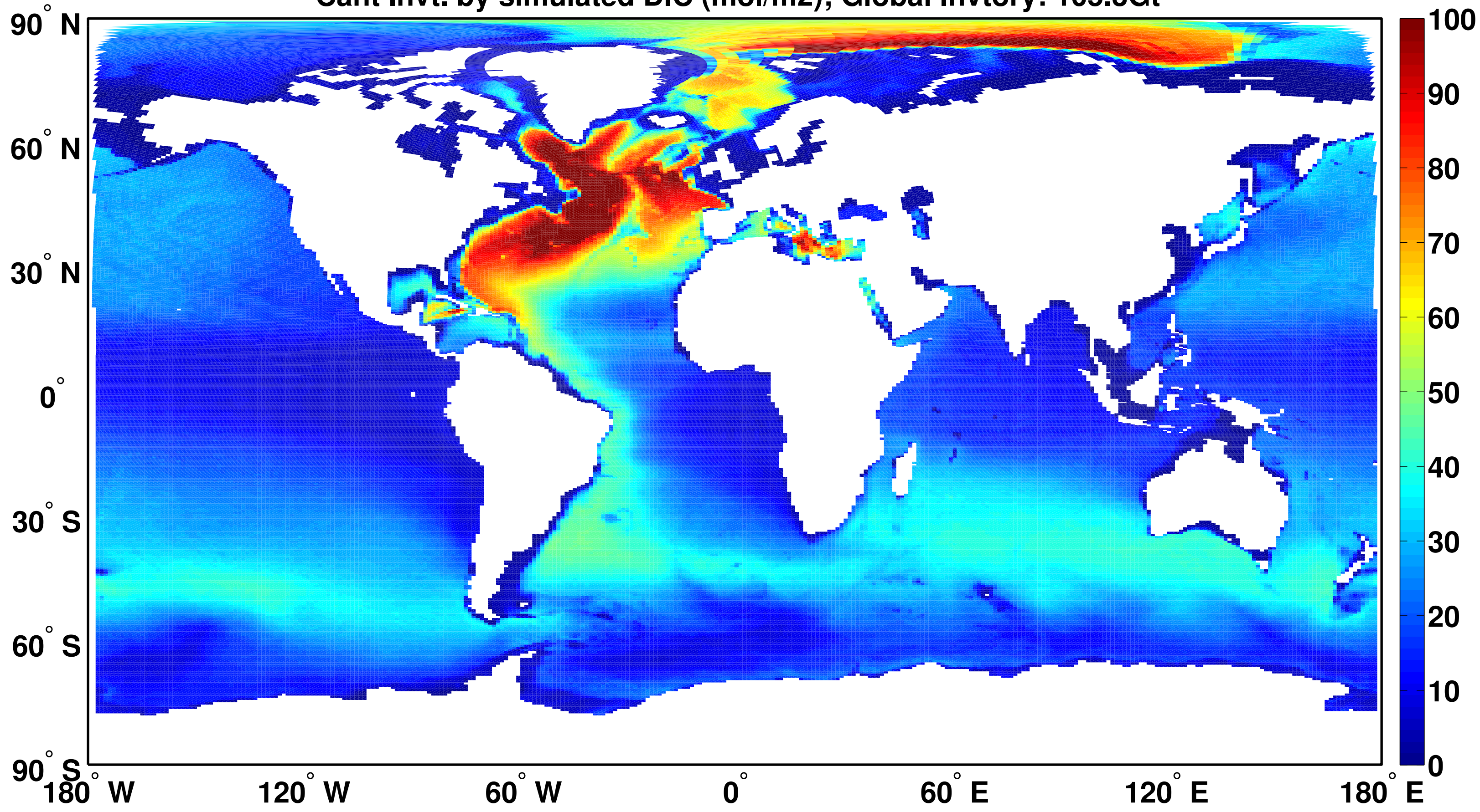
Cant Invt. by simulated DIC (mol/m 2 ); Global Invtory: 105.3Gt
