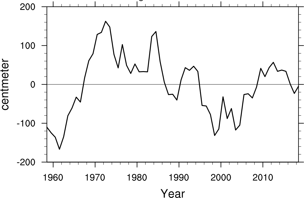
PC3 of Sea Surface Height
