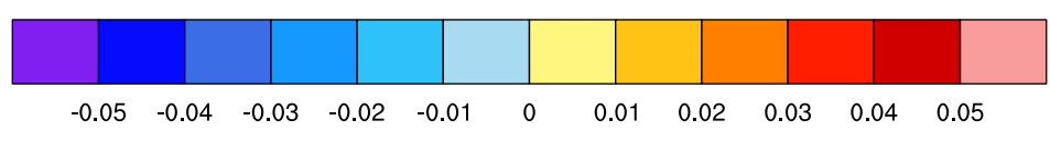
PC2 of Sea Surface Height
