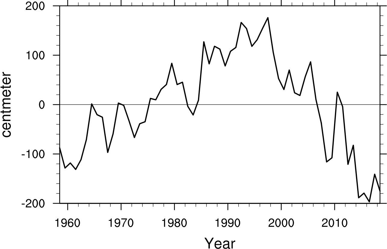
PC2 of Sea Surface Height
