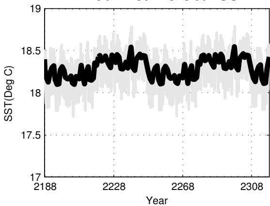
Annual Mean Global SST
