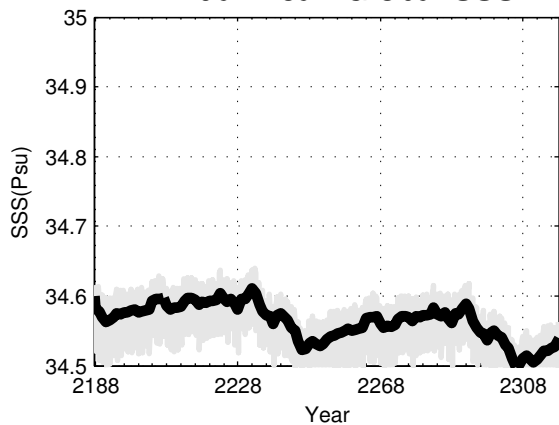
Annual Mean Global SSS
