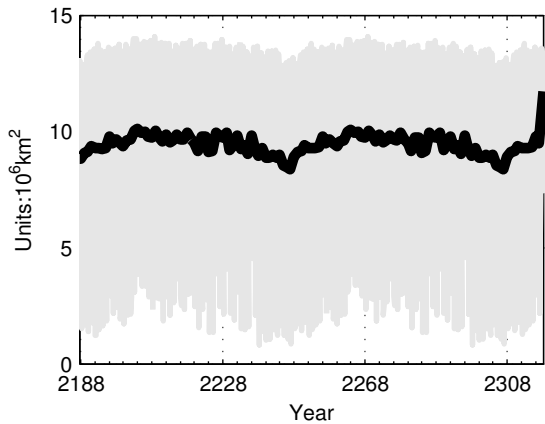
Arctic Sea Ice Area
