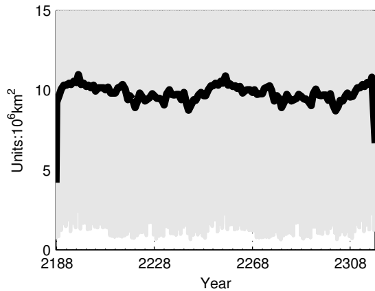
Antarctic Sea Ice Area
