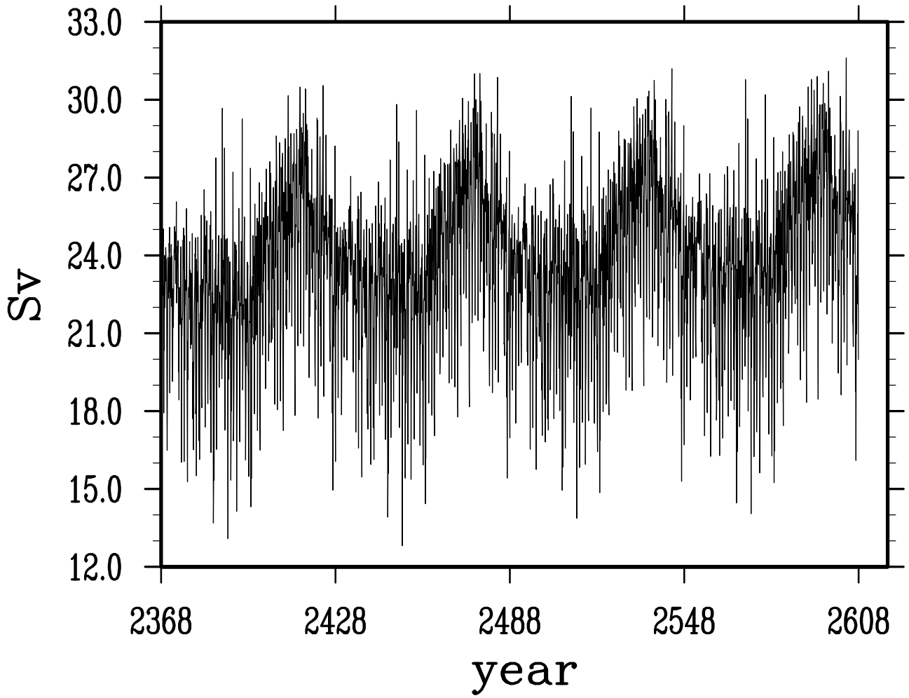
net volume transport across atlantic 41N
