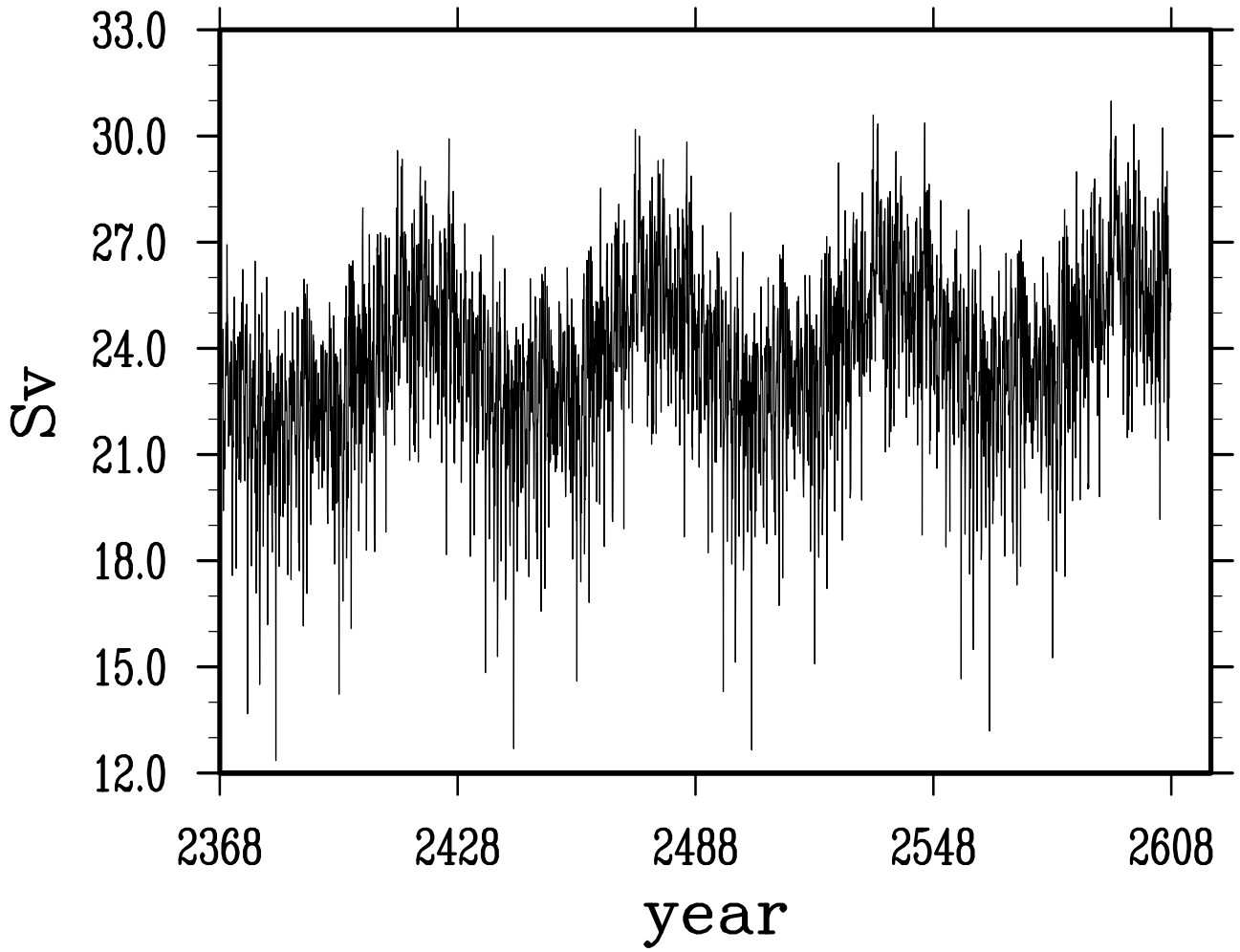
net volume transport across atlantic 26.5N
