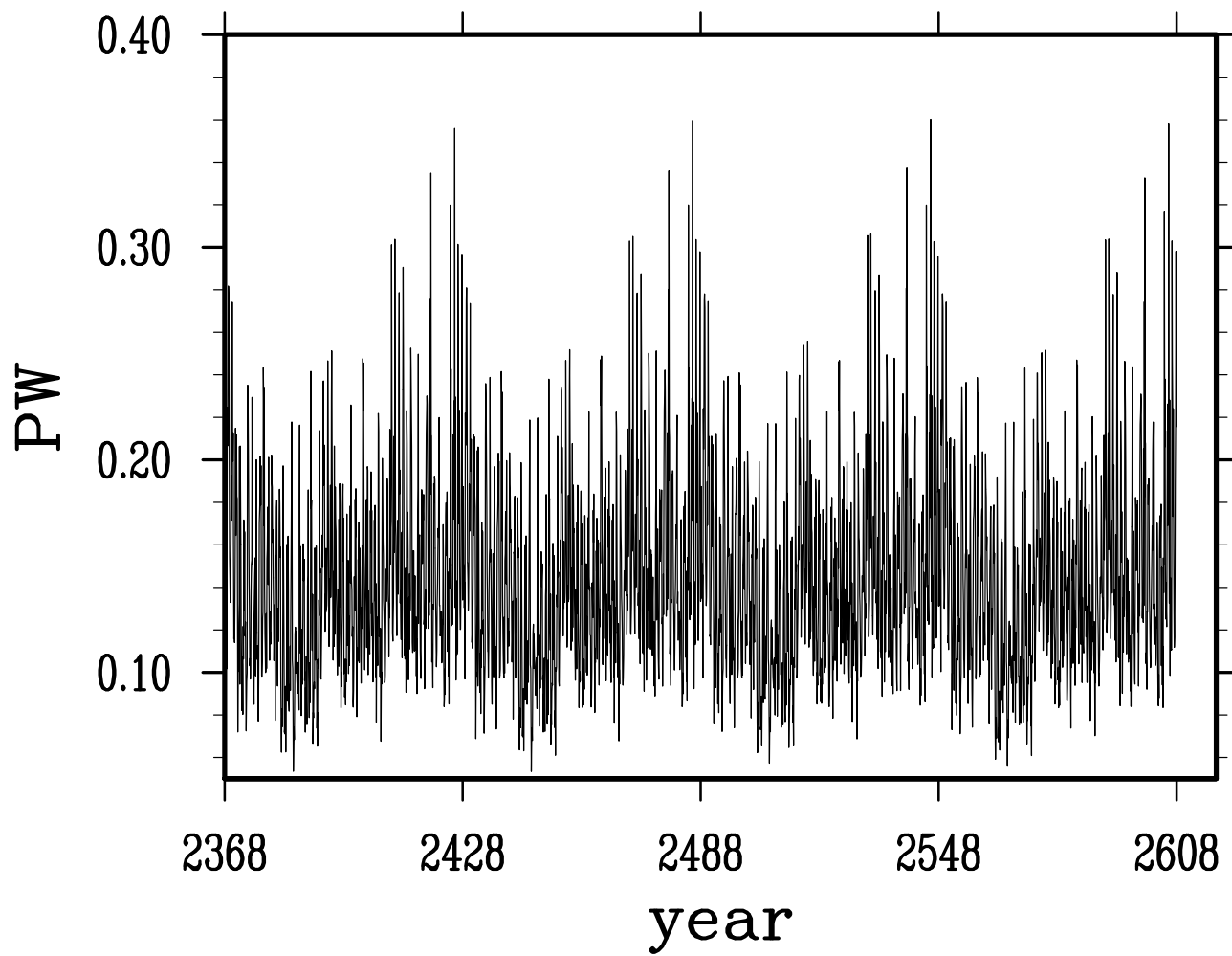
net heat transport across barents opening
