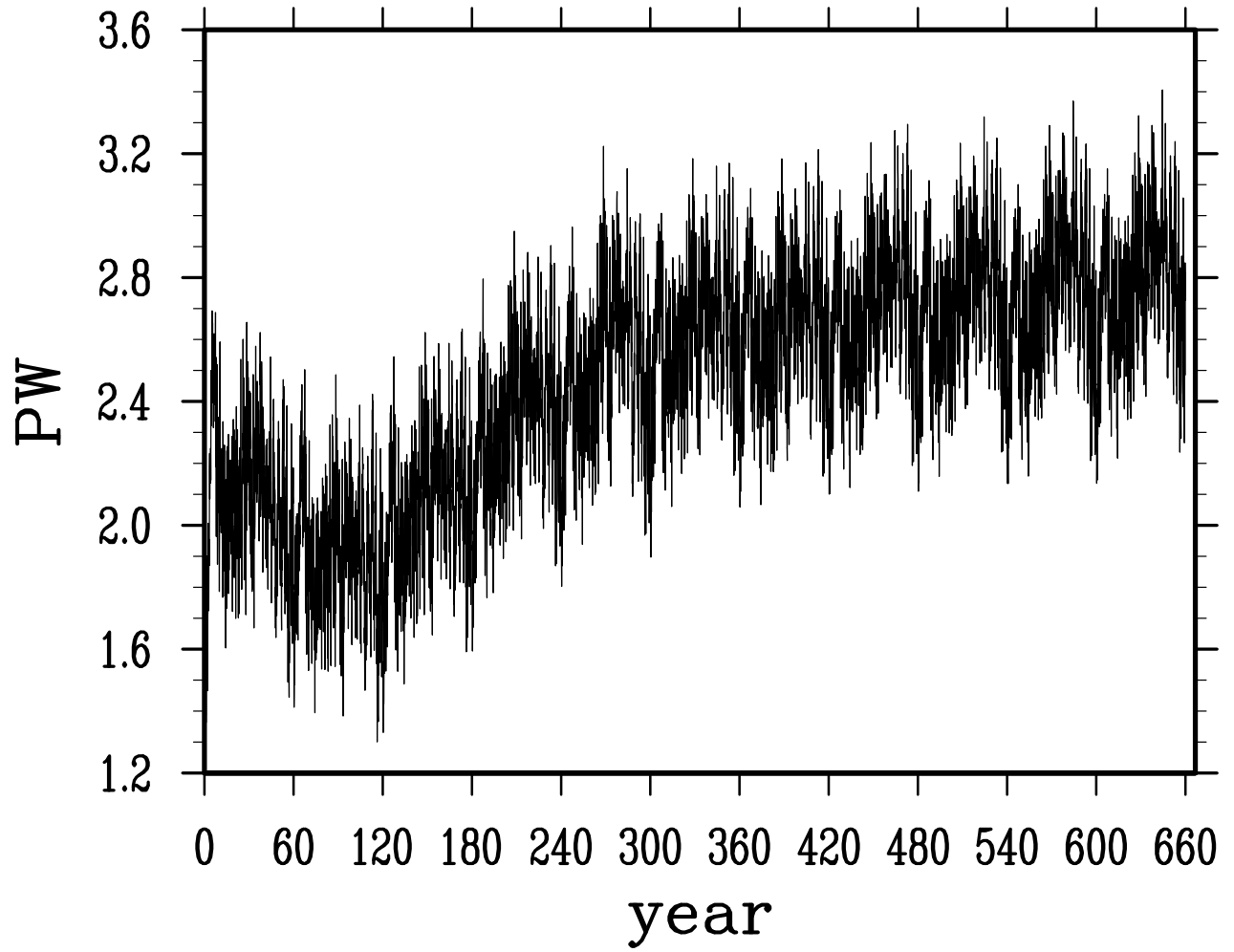
net heat transport across windward passage
