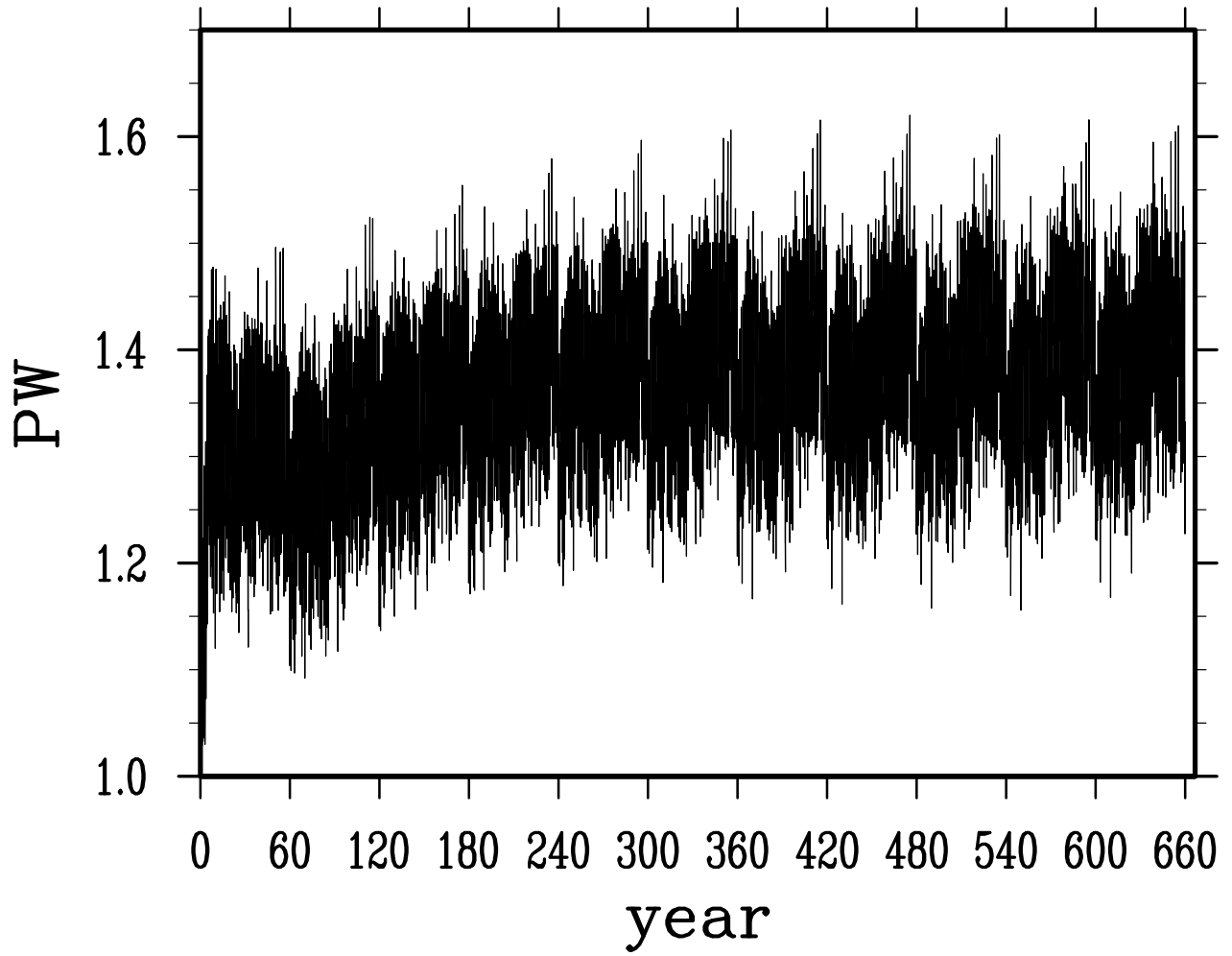
net heat transport across florida bahamas
