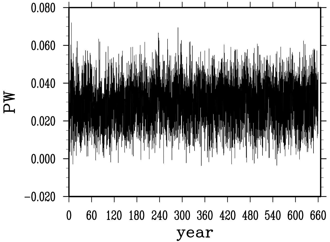
net heat transport across davies strait
