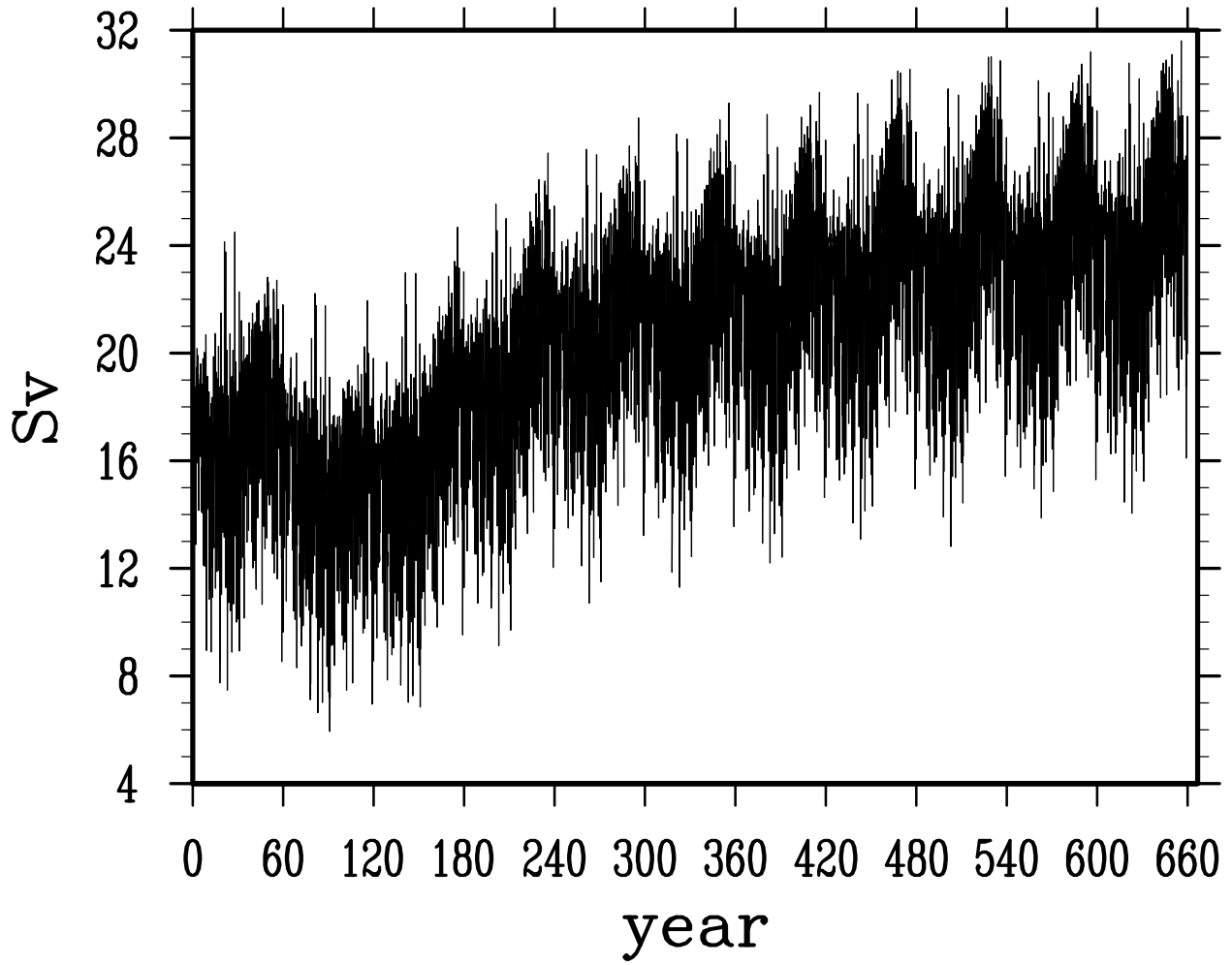
net volume transport across atlantic 41N
