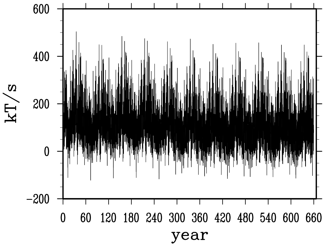
net salt transport across faroe scotland channel
