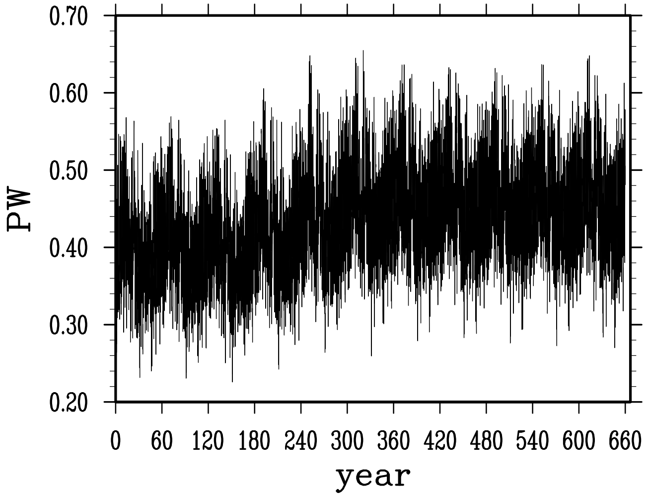
net heat transport across iceland faroe channel
