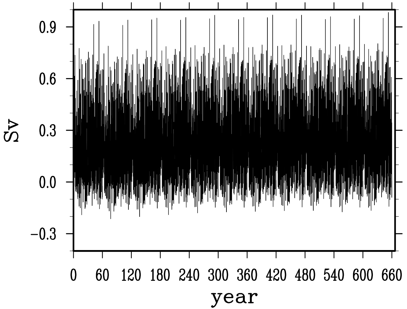
net volume transport across english channel
