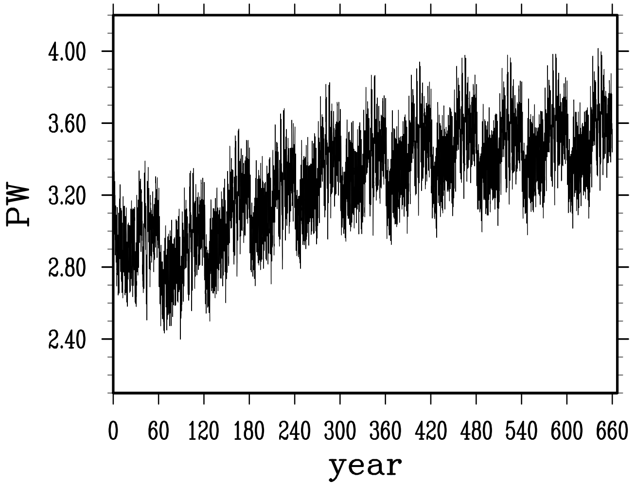
net heat transport across drake passage
