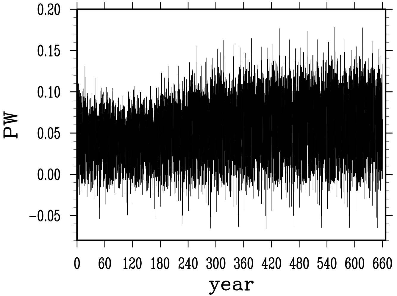
net heat transport across denmark strait
