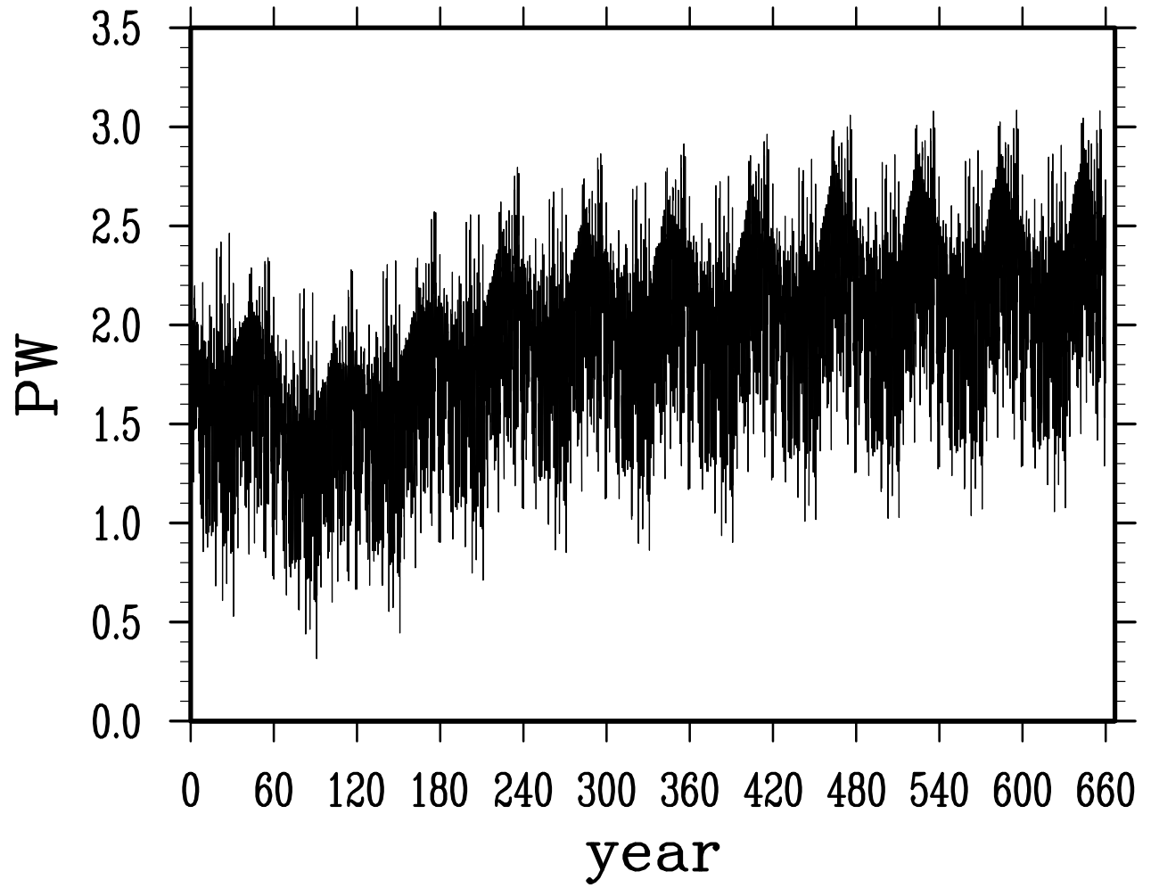
net heat transport across atlantic 41N
