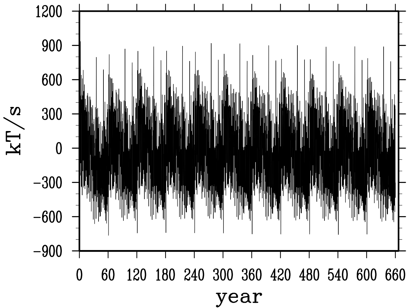
net salt transport across taiwan and luzon straits
