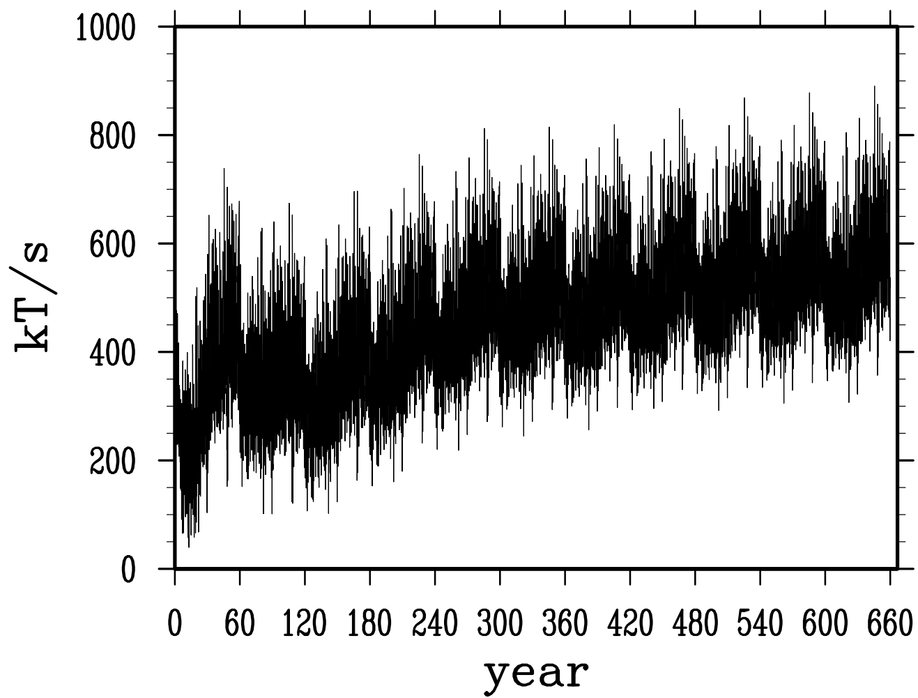
net salt transport across atlantic 30S
