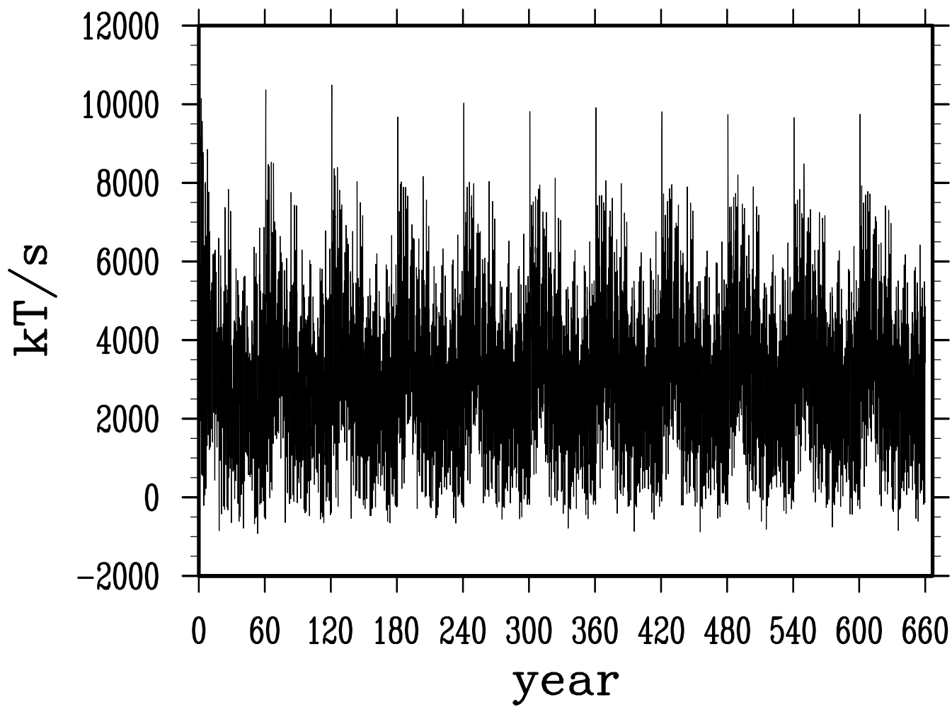
net salt transport across equatorial undercurrent
