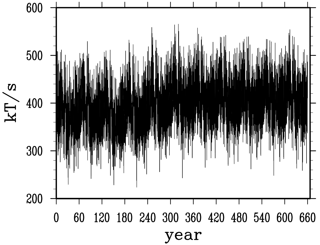
net salt transport across iceland faroe channel
