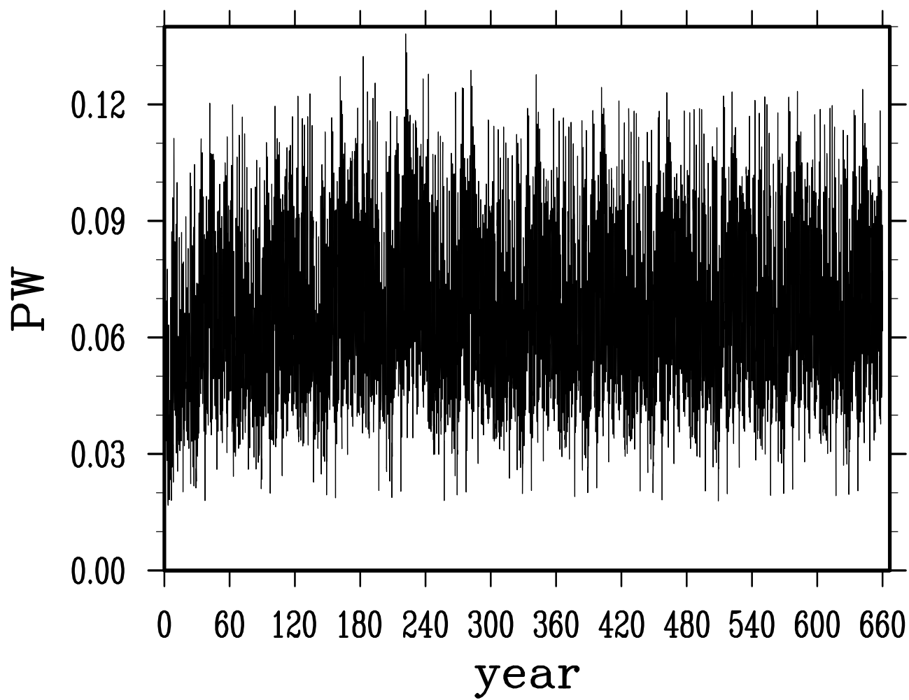
net heat transport across fram strait
