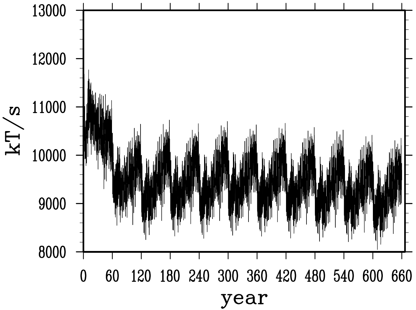
net salt transport across drake passage
