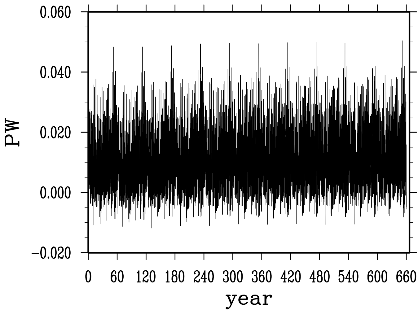
net heat transport across english channel
