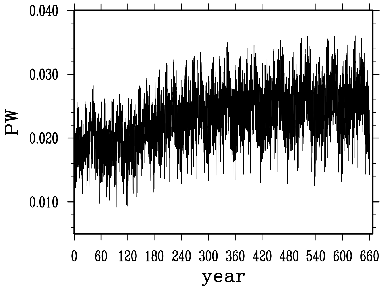
net heat transport across canadian archipelago
