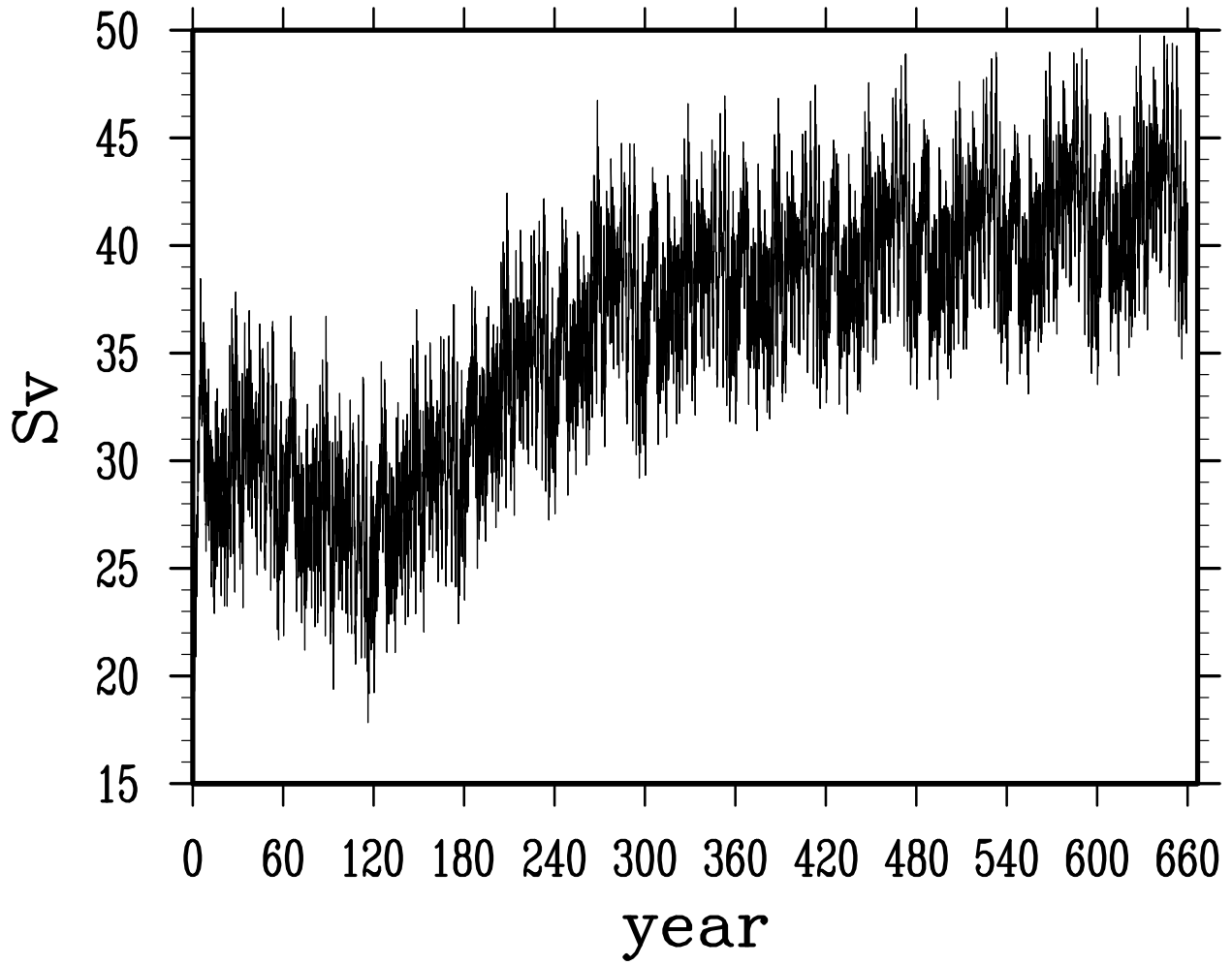
net volume transport across windward passage
