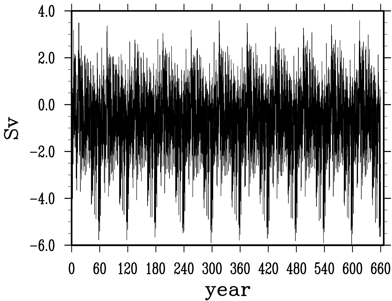
net volume transport across fram strait
