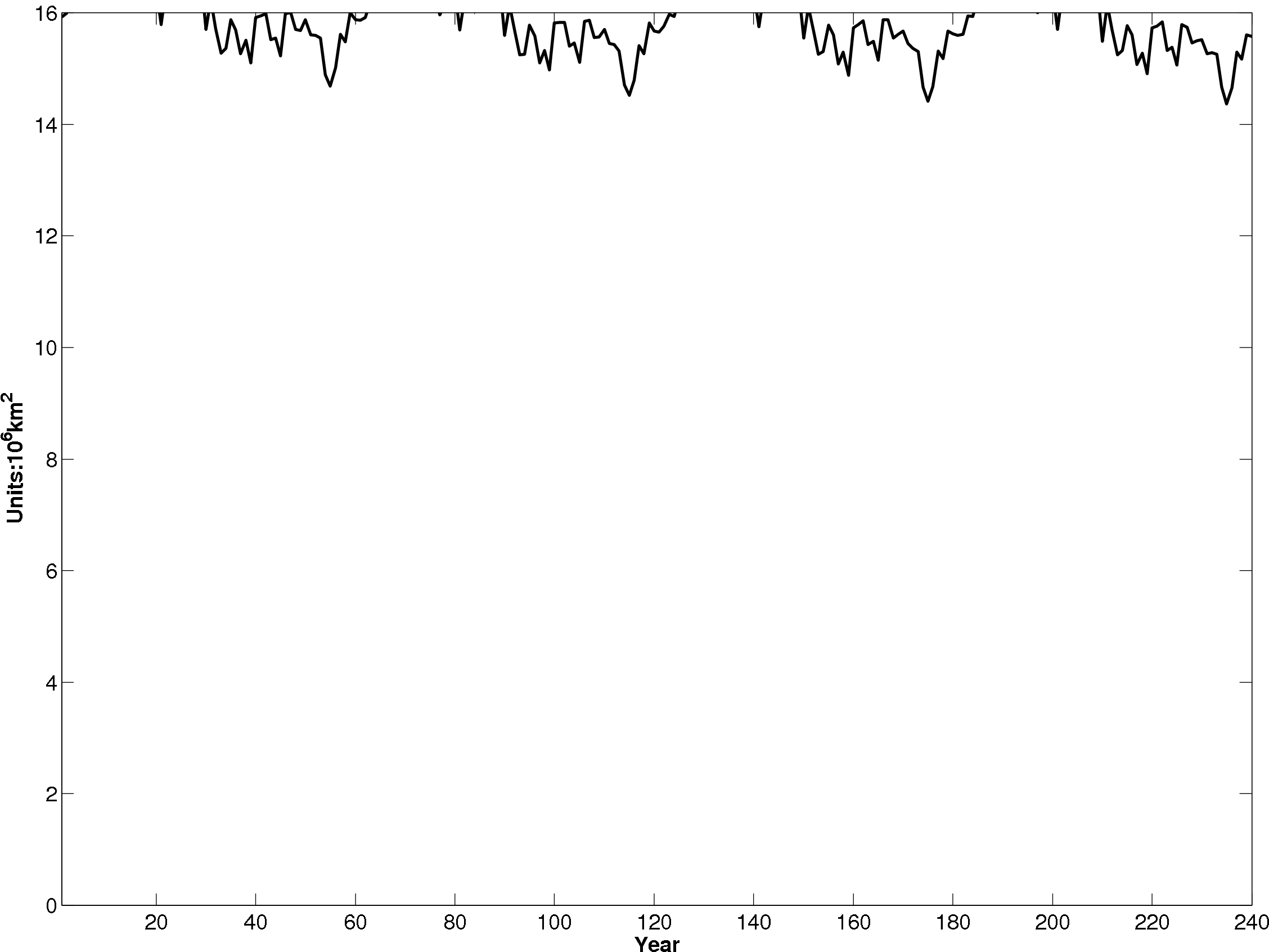
Antarctic Sea Ice Area
