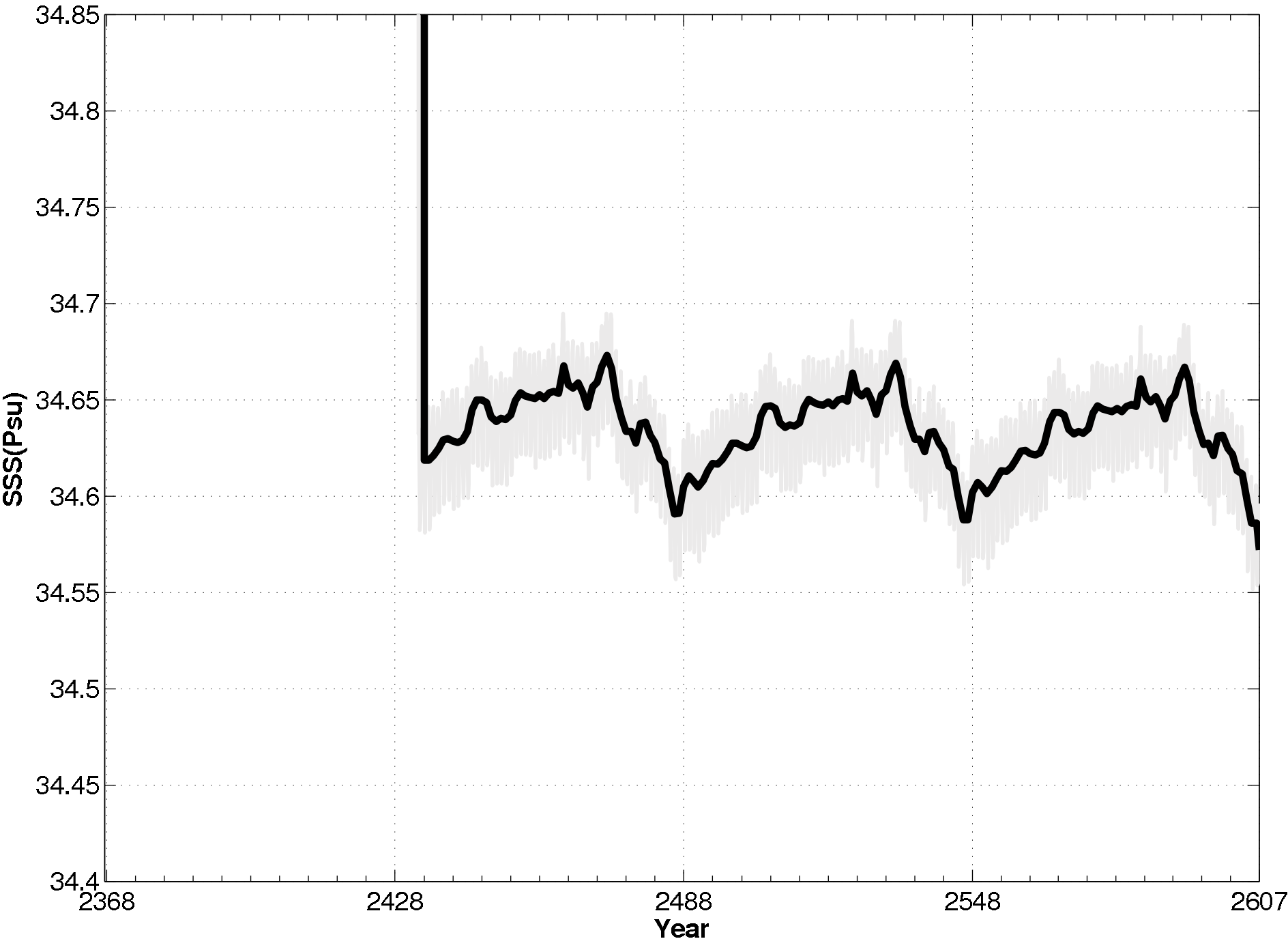
Annual Mean Global SSS
