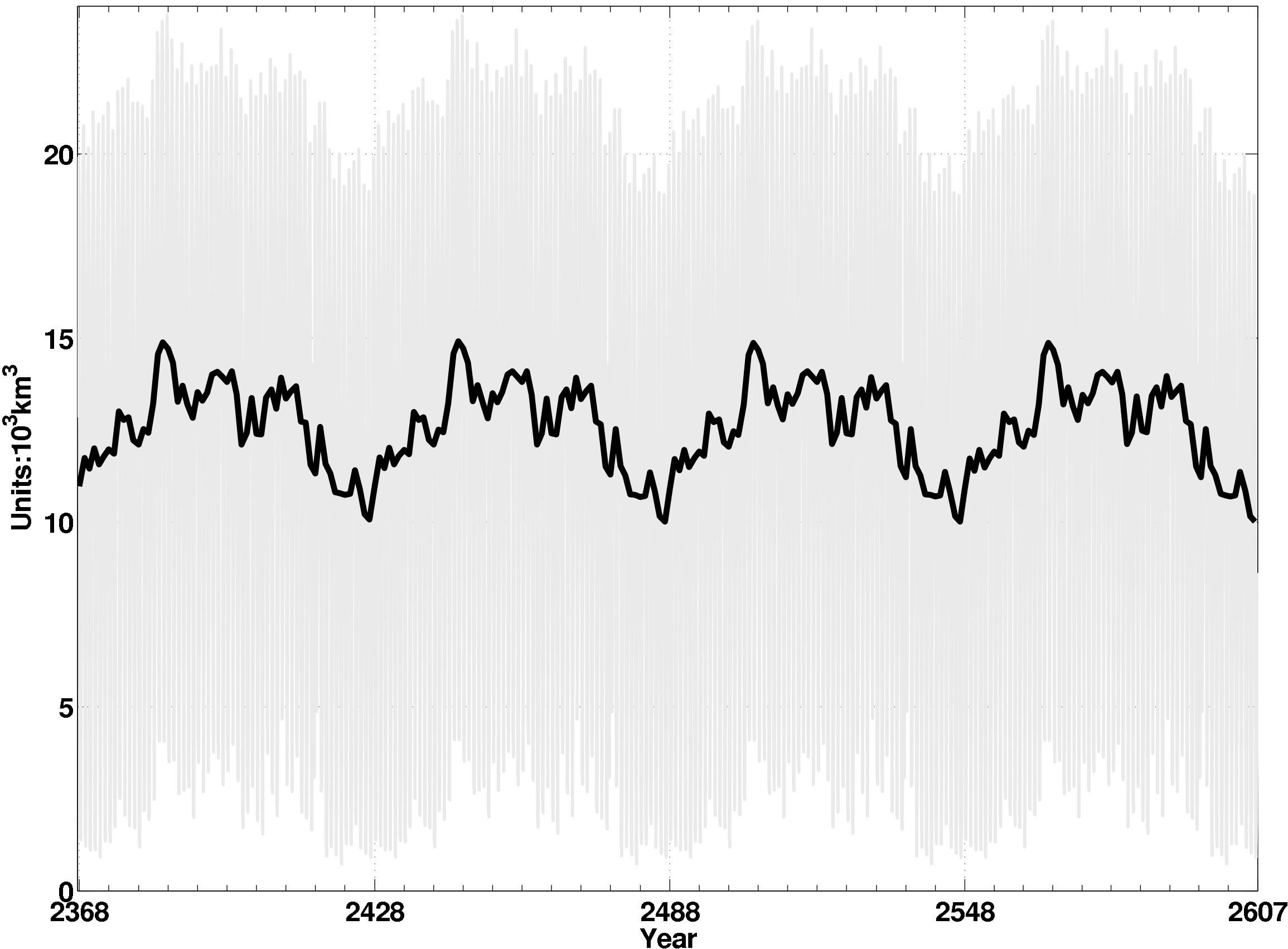
Arctic Sea Ice Volume (thickness)
