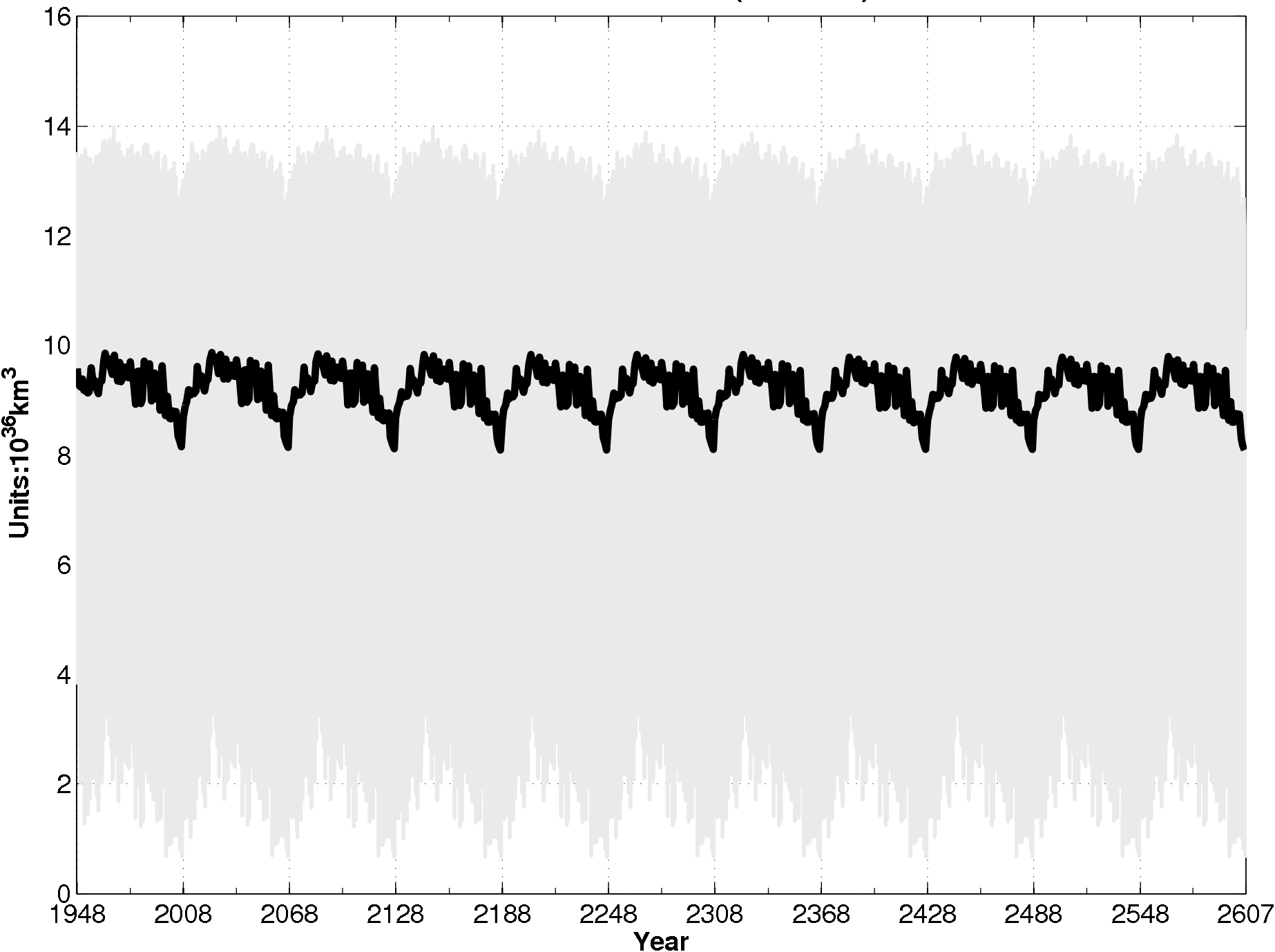
Arctic Sea Ice Volume (thickness)
