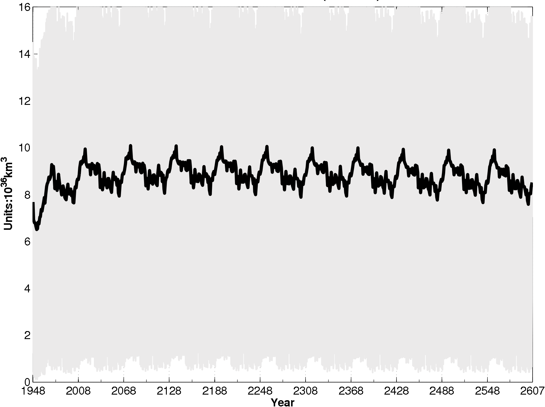
Antarctic Sea Ice Volume (thickness)
