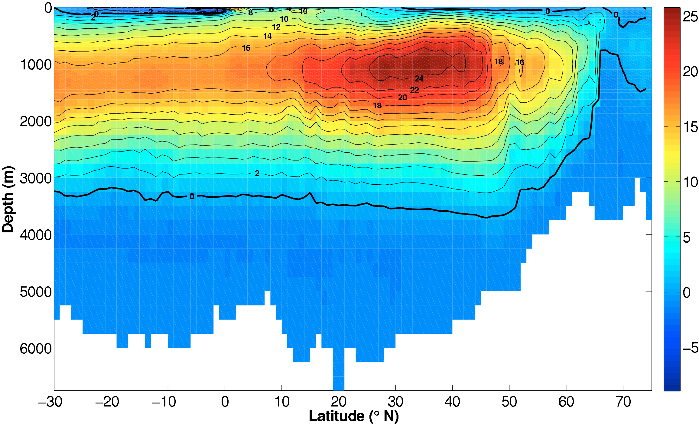
Longterm Mean Atlantic Meridional Overturning Stream Function
