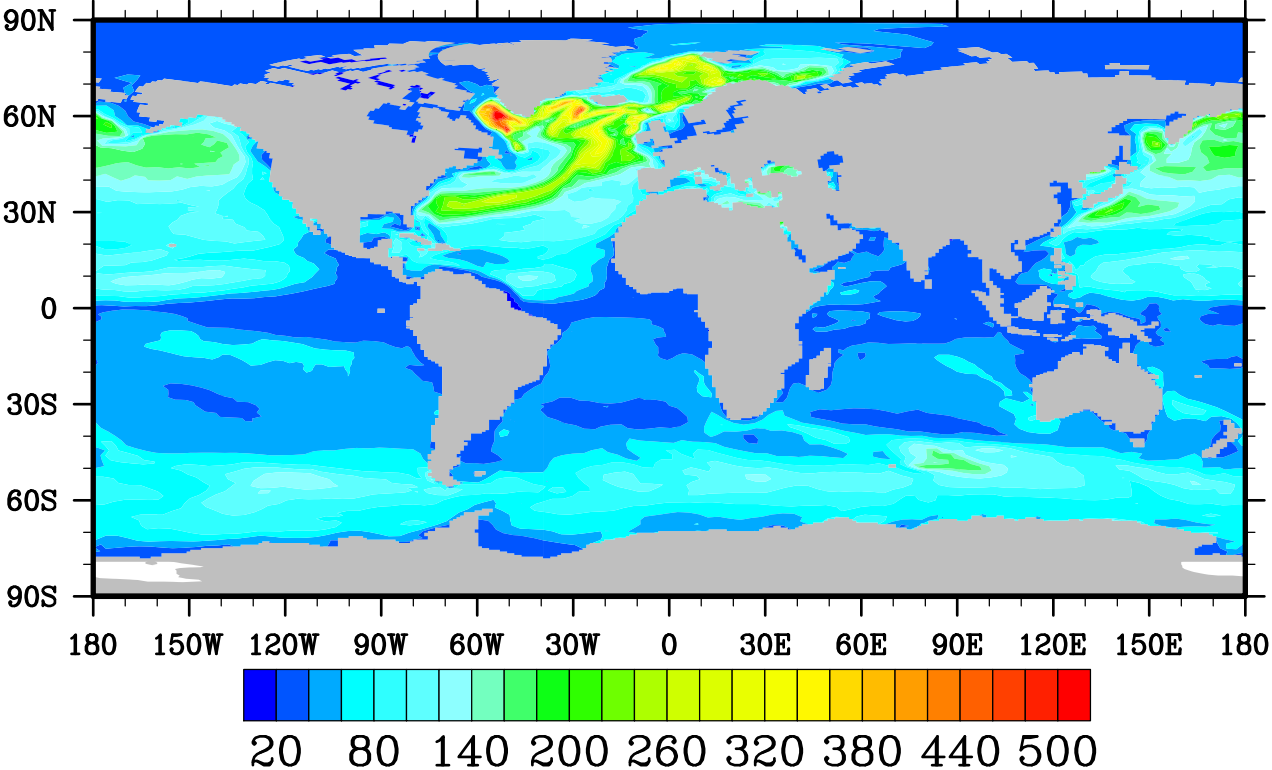
Mean of Sept. MXLD (last 240yrs)
