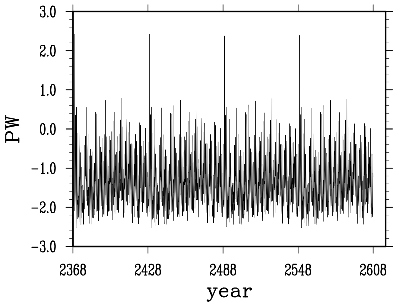
net heat transport across indonesian throughflow
