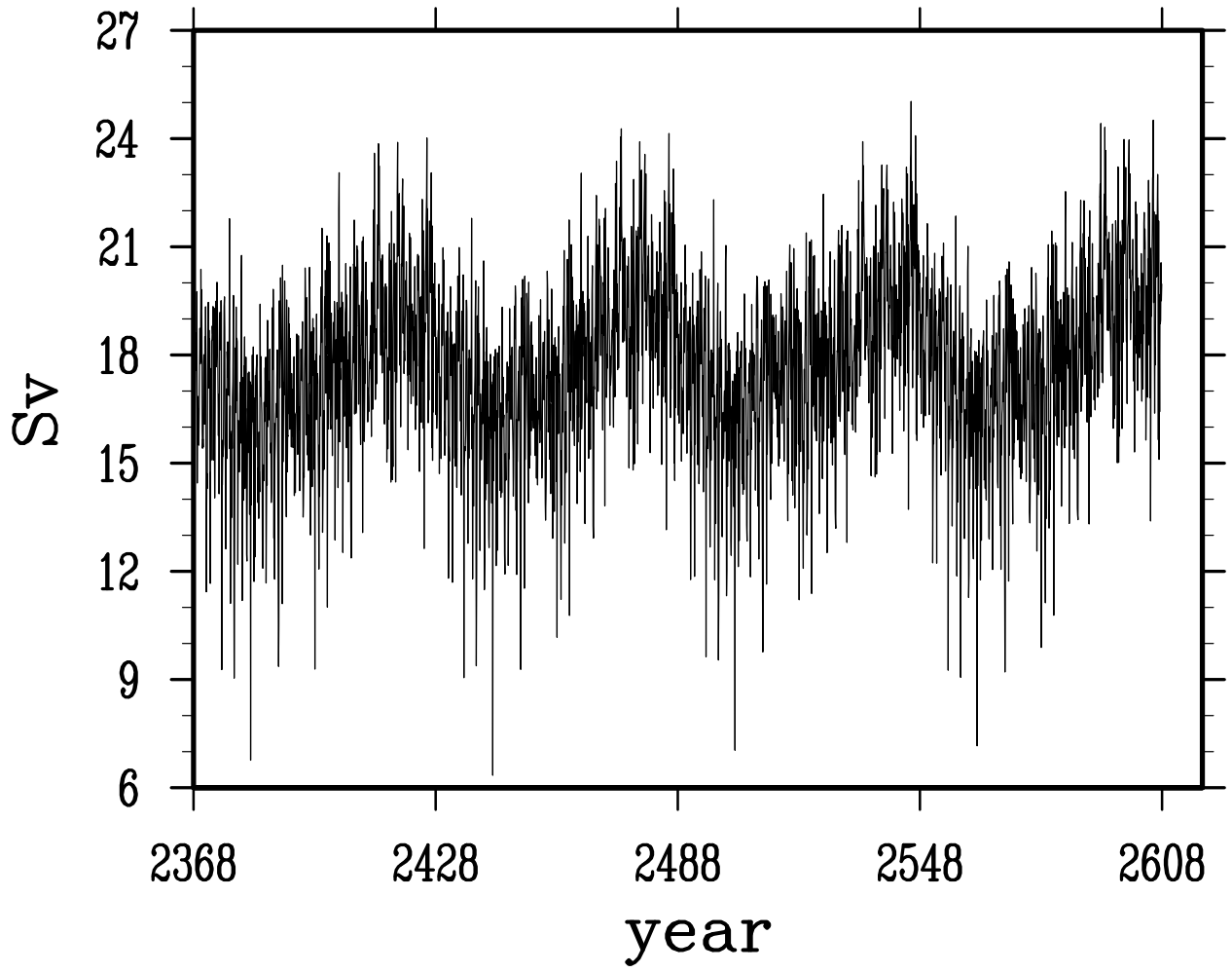
net volume transport across atlantic 26.5N
