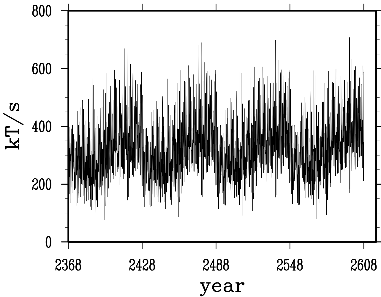
net salt transport across atlantic 30S
