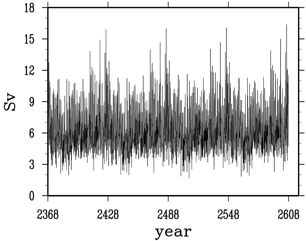
net volume transport across barents opening
