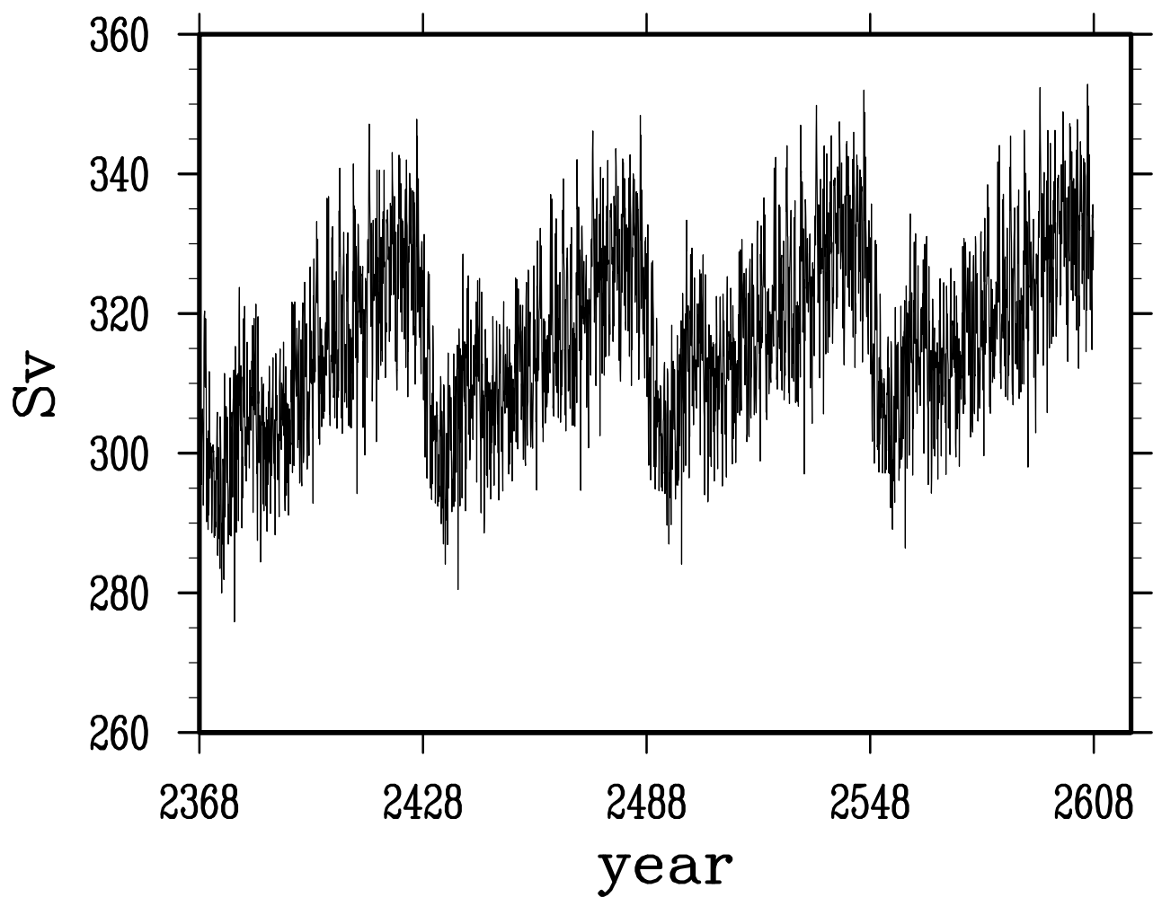
net volume transport across drake passage
