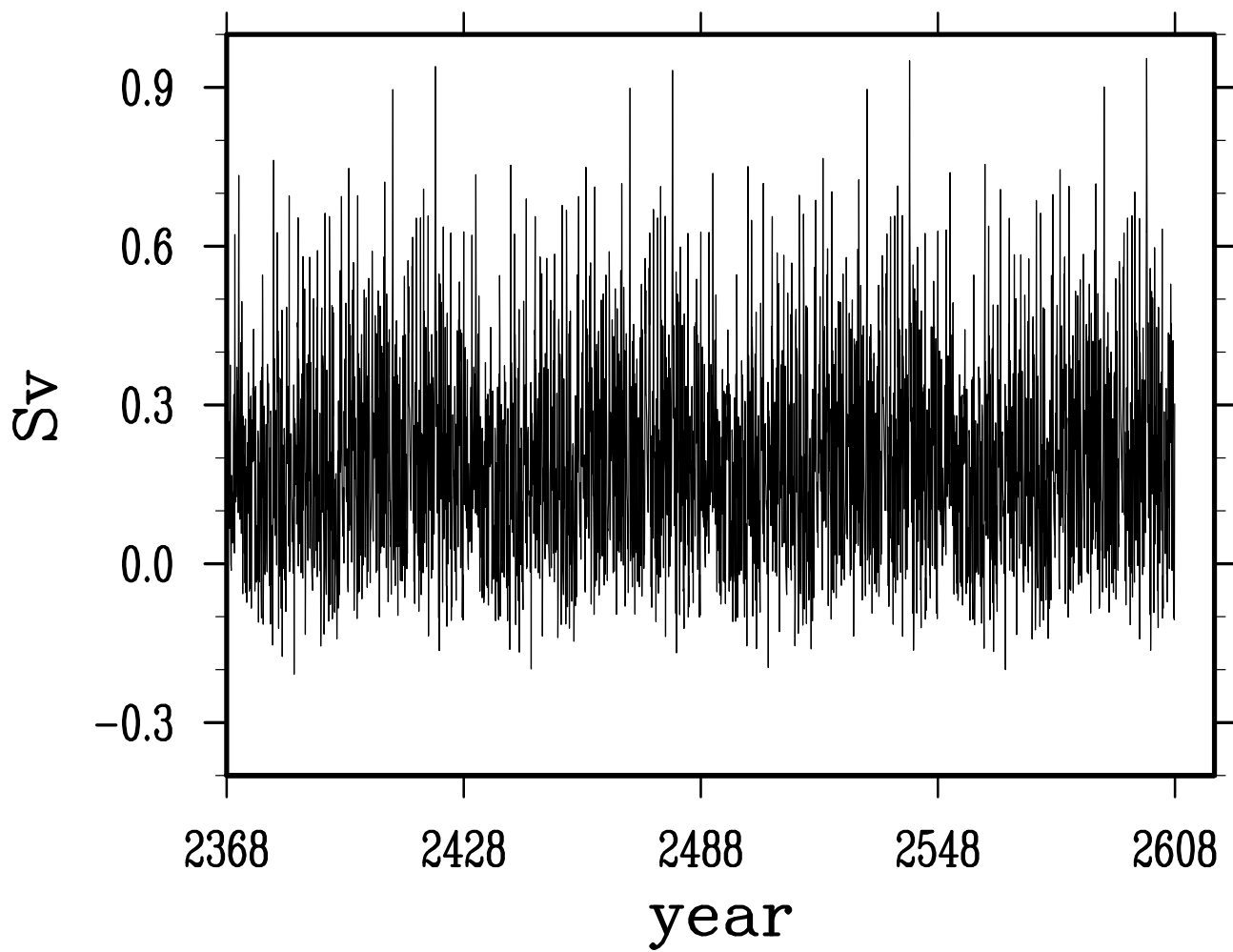
net volume transport across english channel
