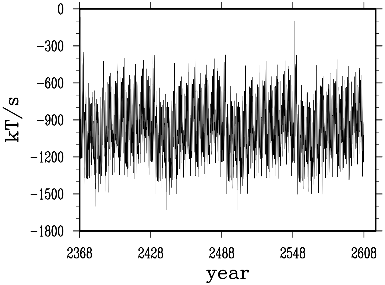
net salt transport across mozambique channel
