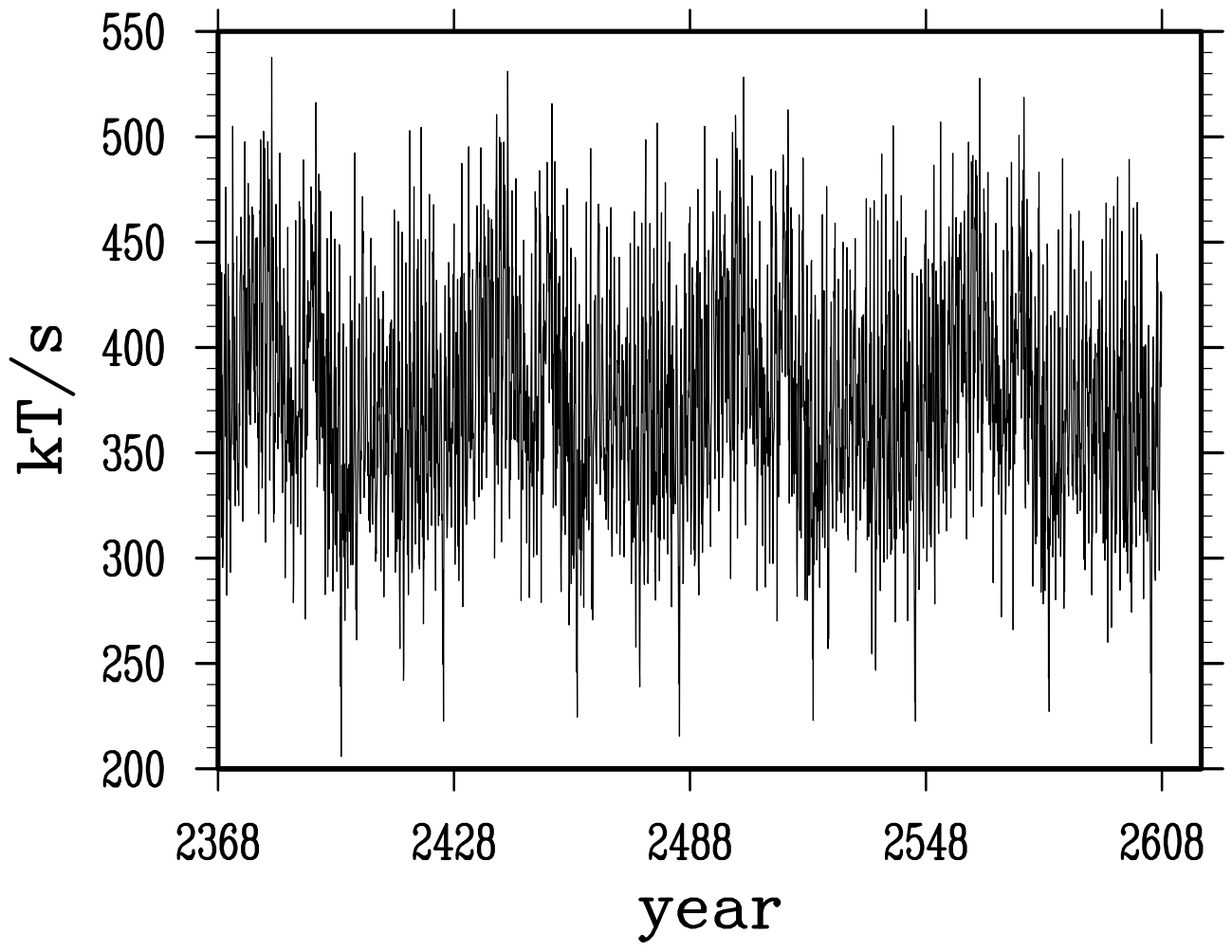
net salt transport across iceland faroe channel
