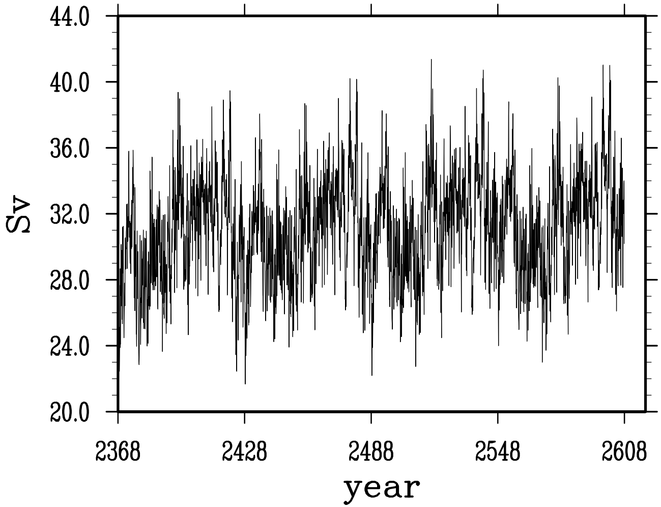
net volume transport across windward passage
