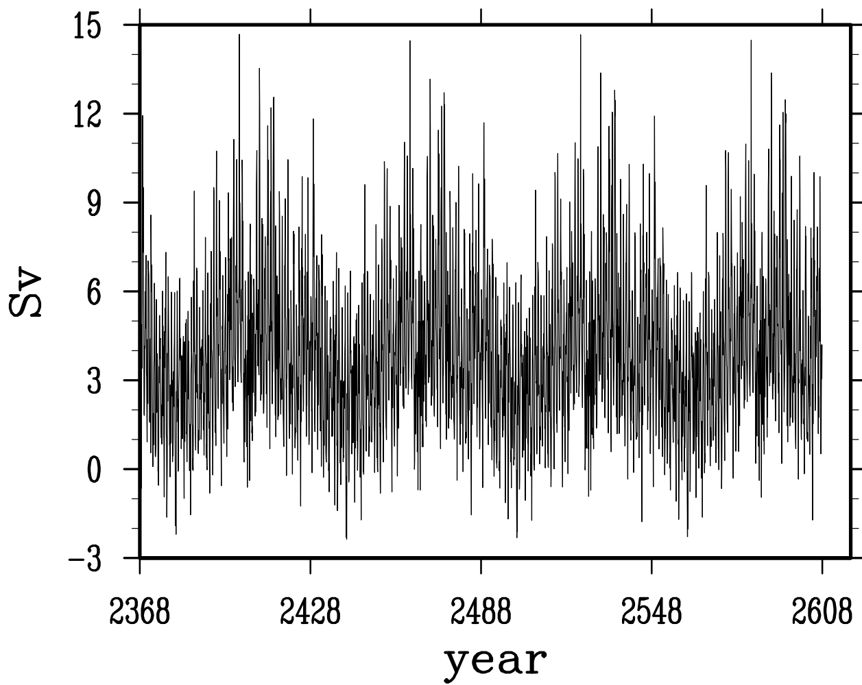
net volume transport across faroe scotland channel
