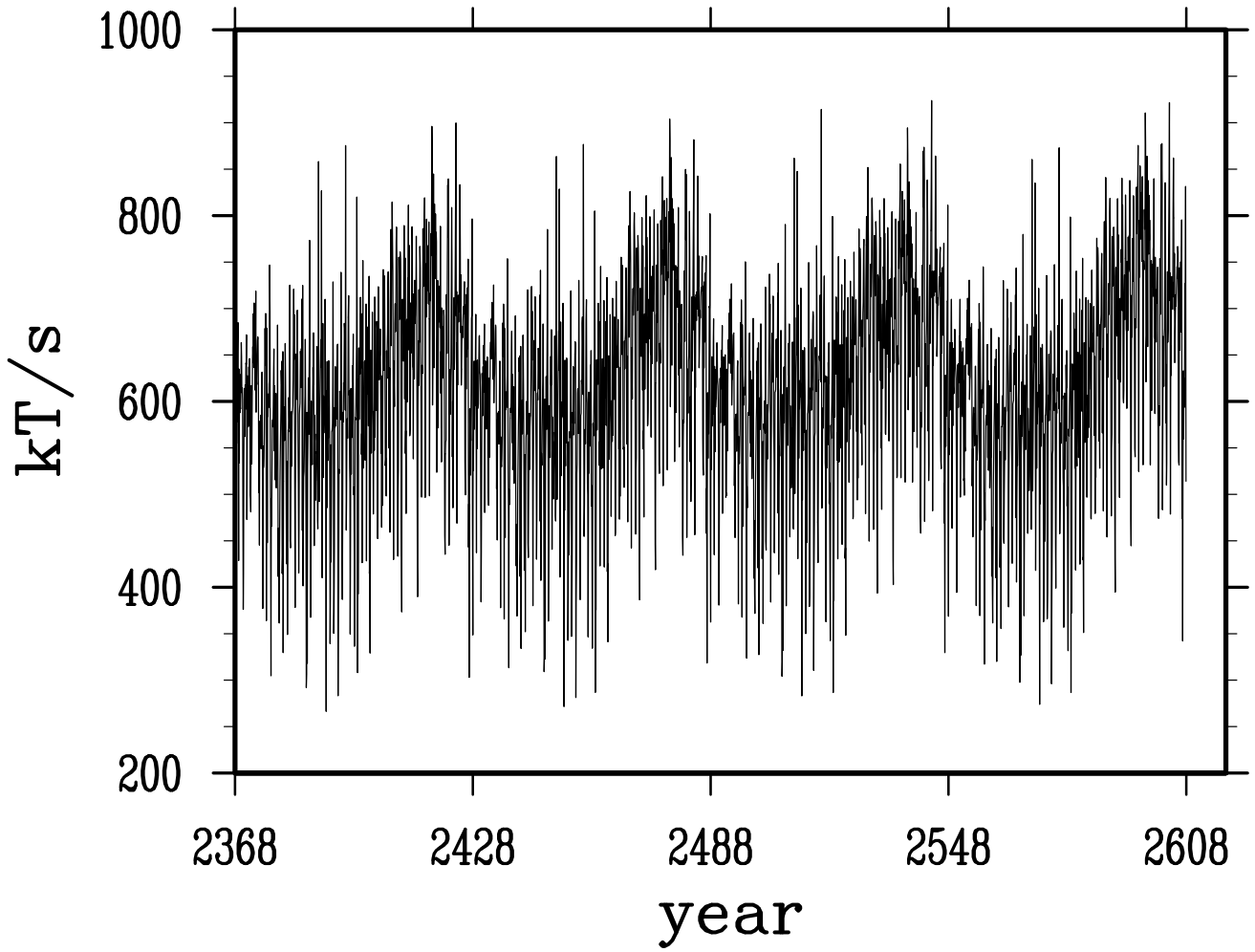
net salt transport across atlantic 41N
