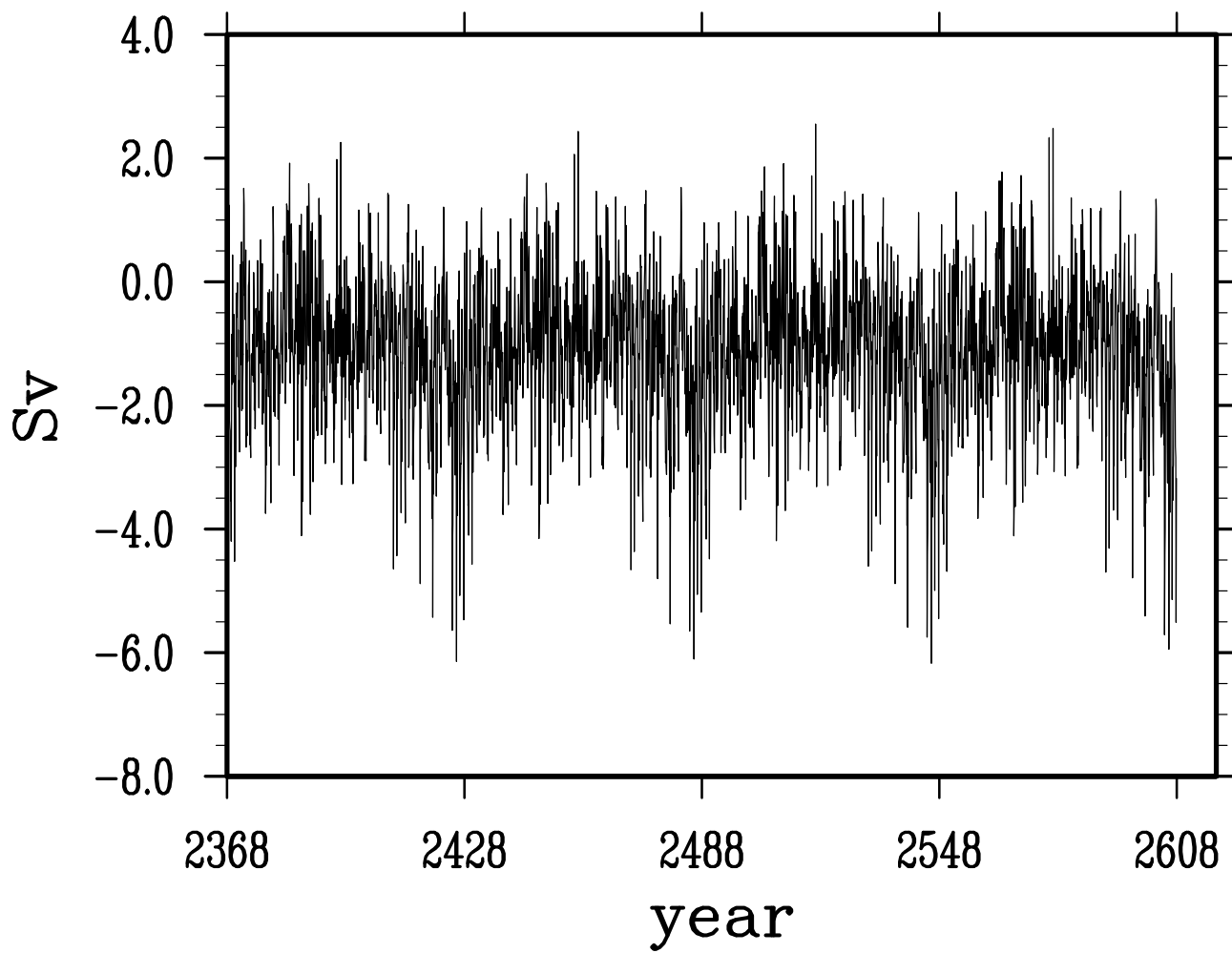
net volume transport across fram strait
