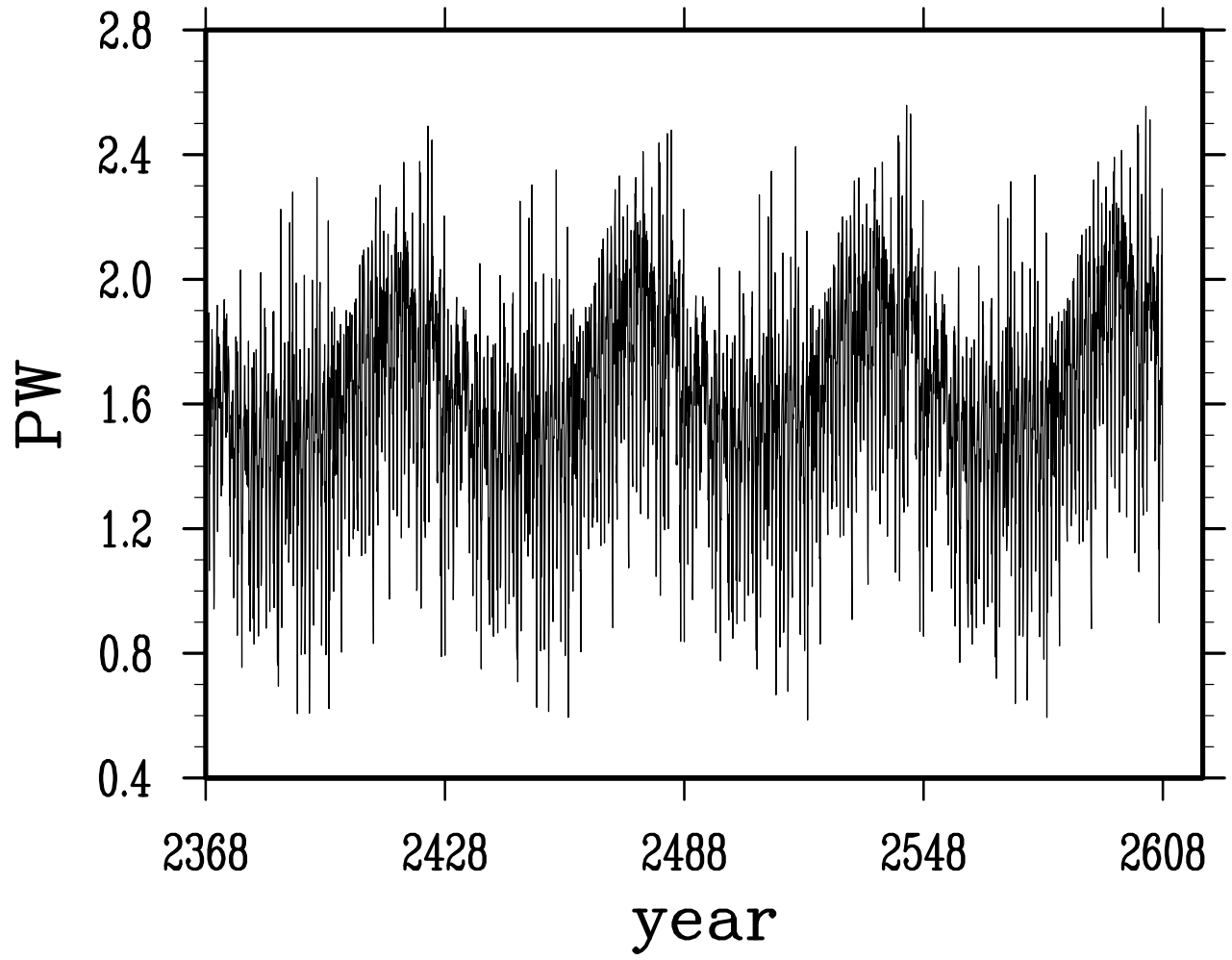
net heat transport across atlantic 41N
