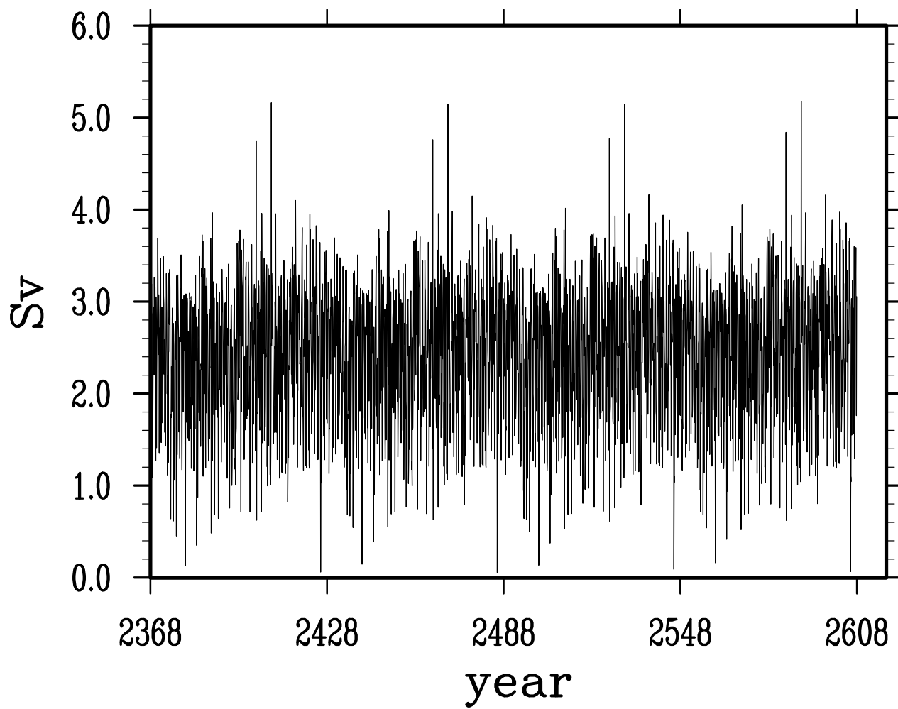
net volume transport across bering strait
