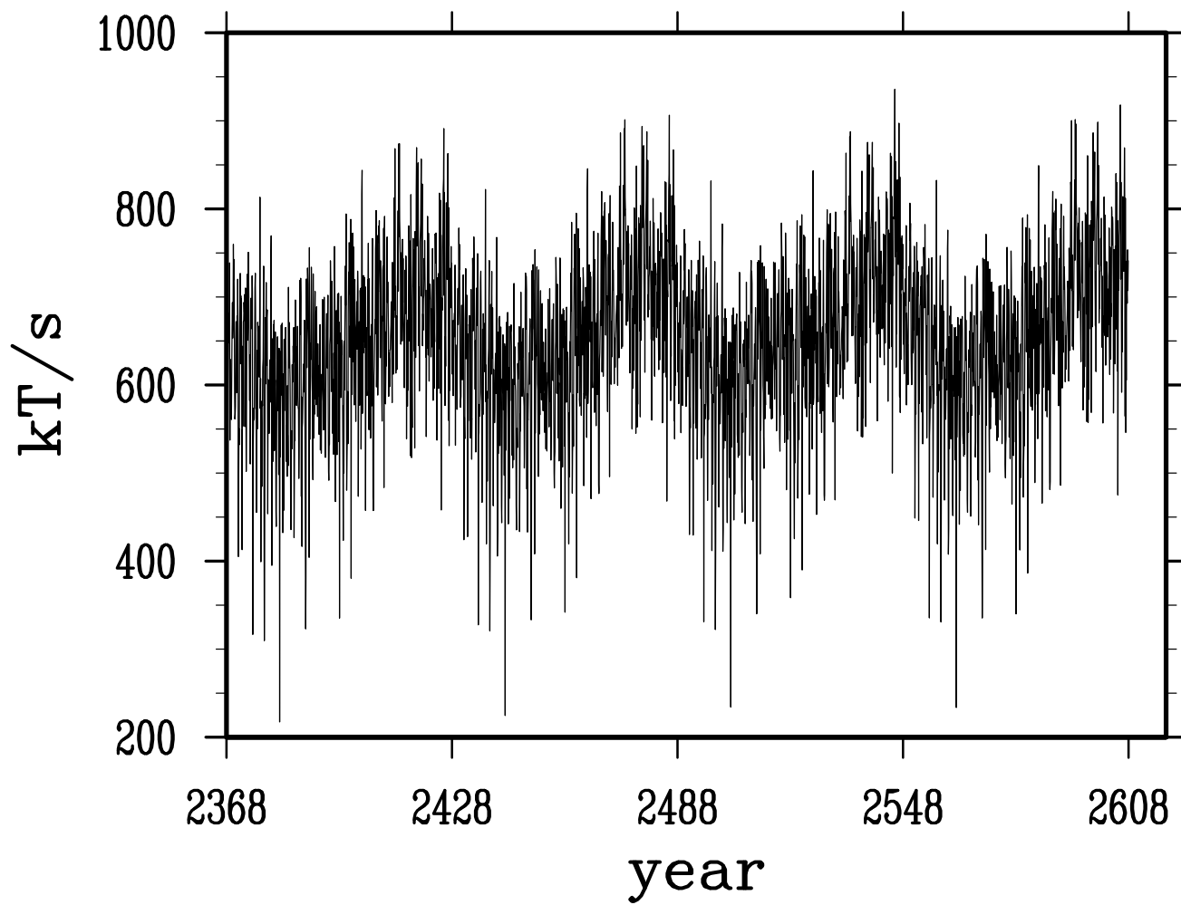
net salt transport across atlantic 26.5N
