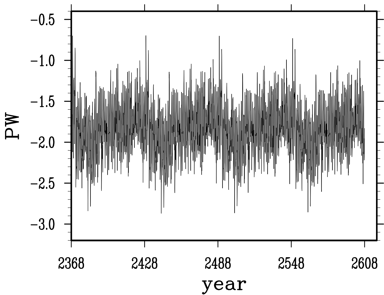
net heat transport across mozambique channel
