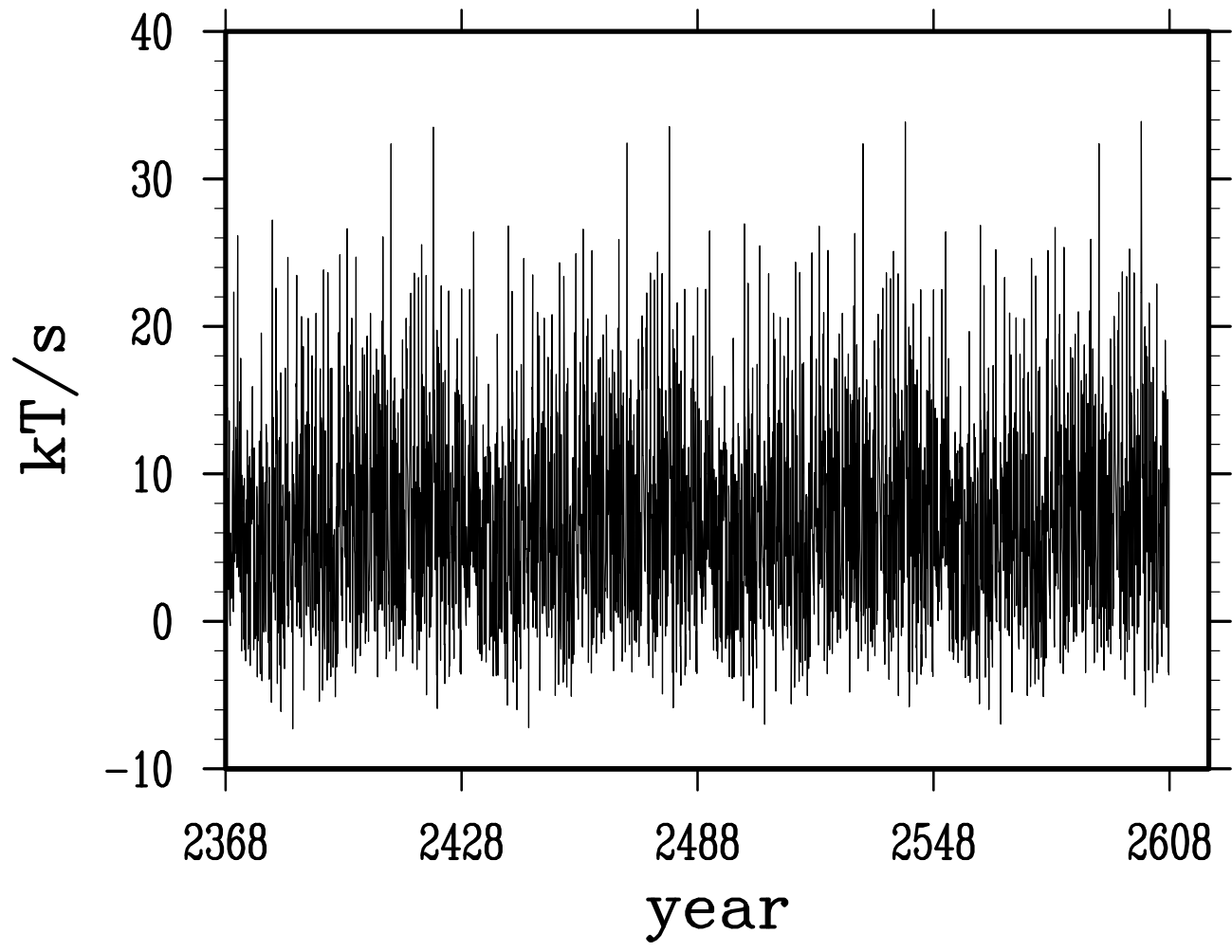
net salt transport across english channel
