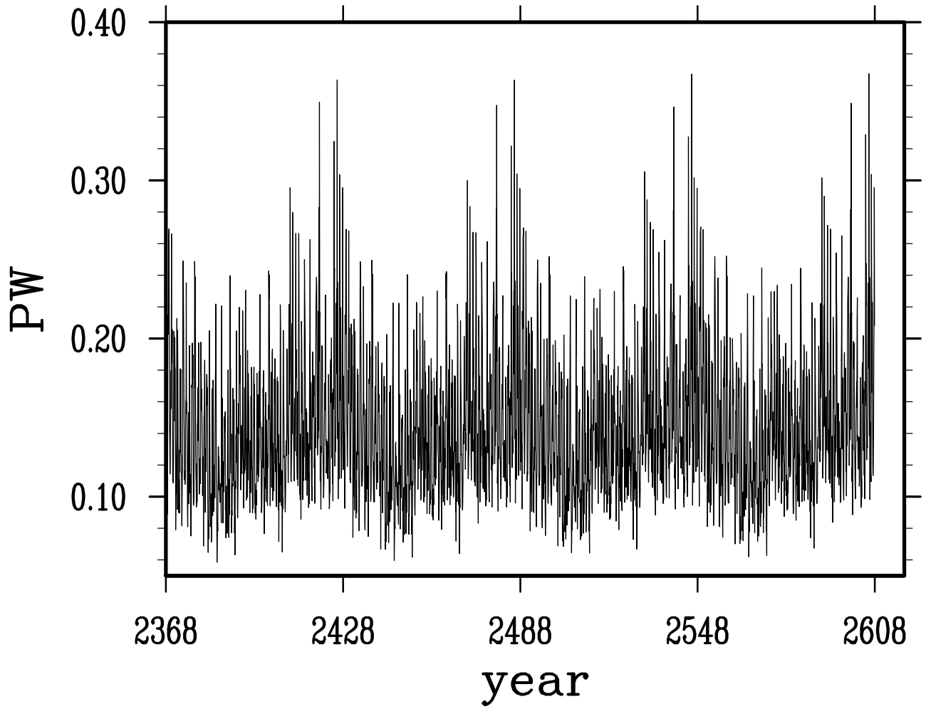
net heat transport across barents opening
