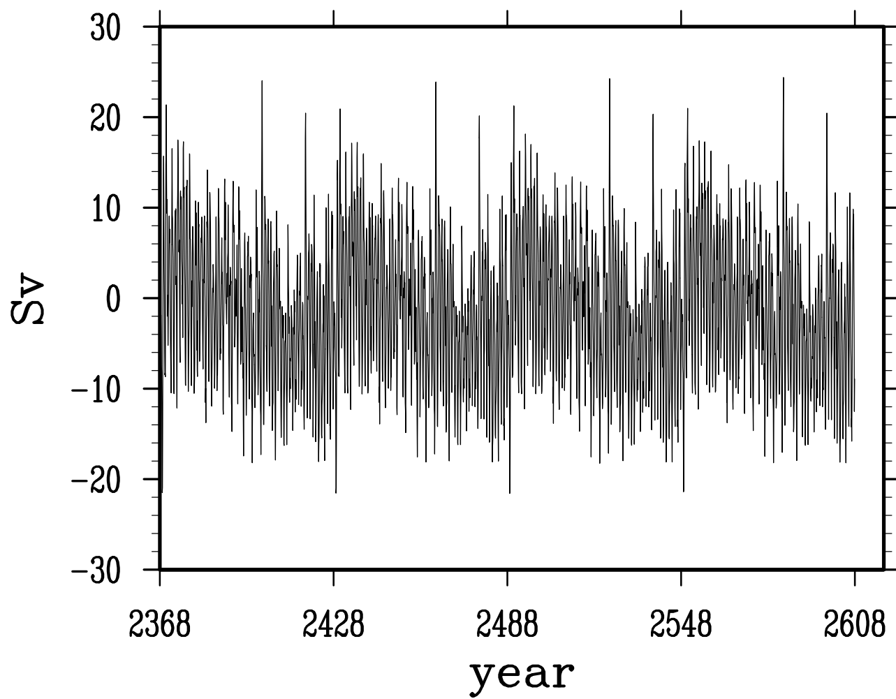
net volume transport across taiwan and luzon straits
