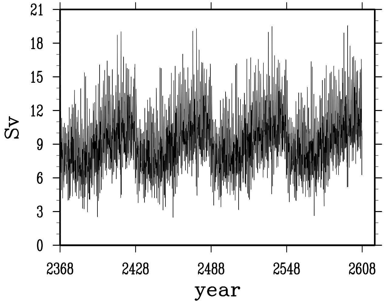
net volume transport across atlantic 30S
