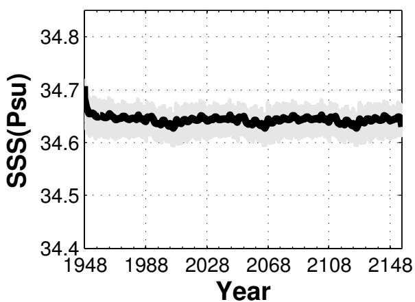
Annual Mean Global SSS
