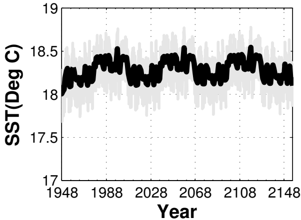
Annual Mean Global SST
