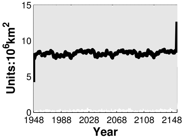
Antarctic Sea Ice Area
