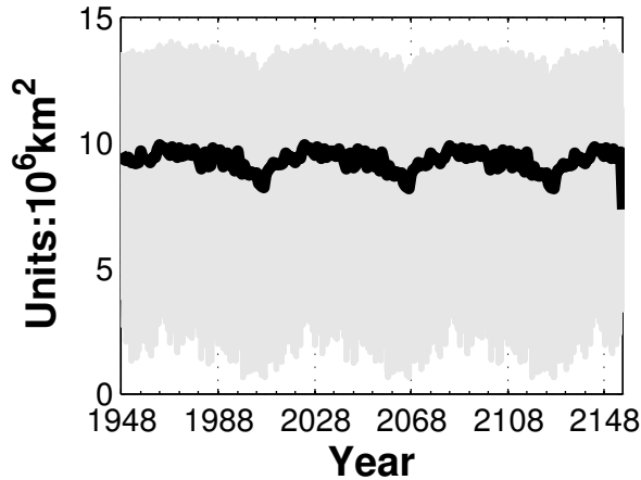
Arctic Sea Ice Area
