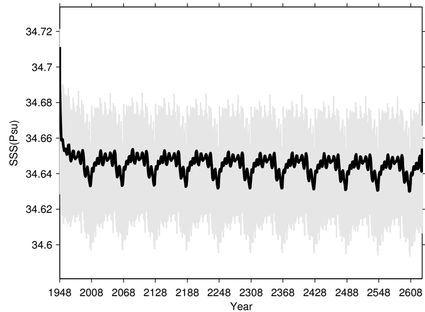
Annual Mean Global SSS
