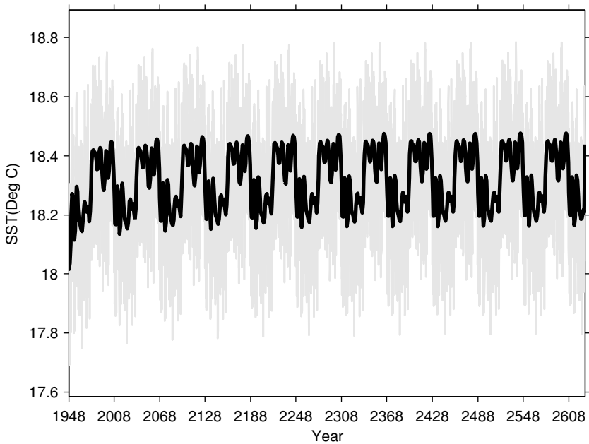
Annual Mean Global SST
