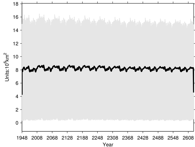
Antarctic Sea Ice Area
