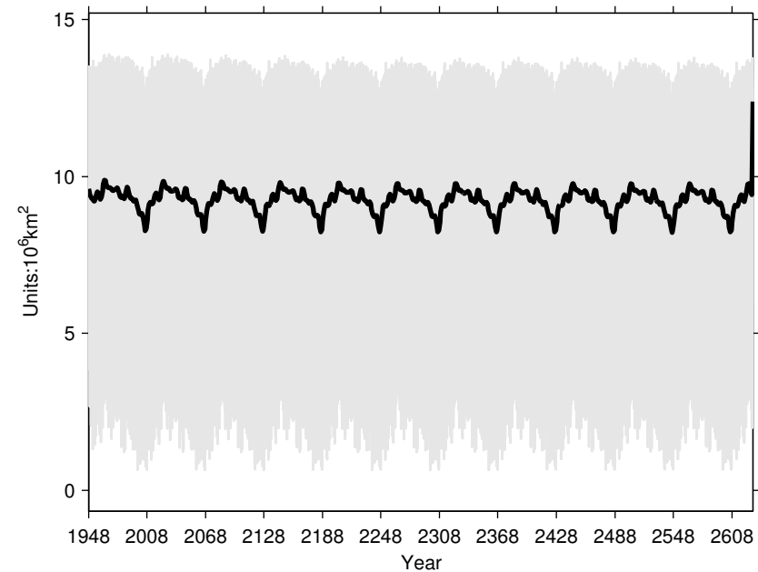
Arctic Sea Ice Area
