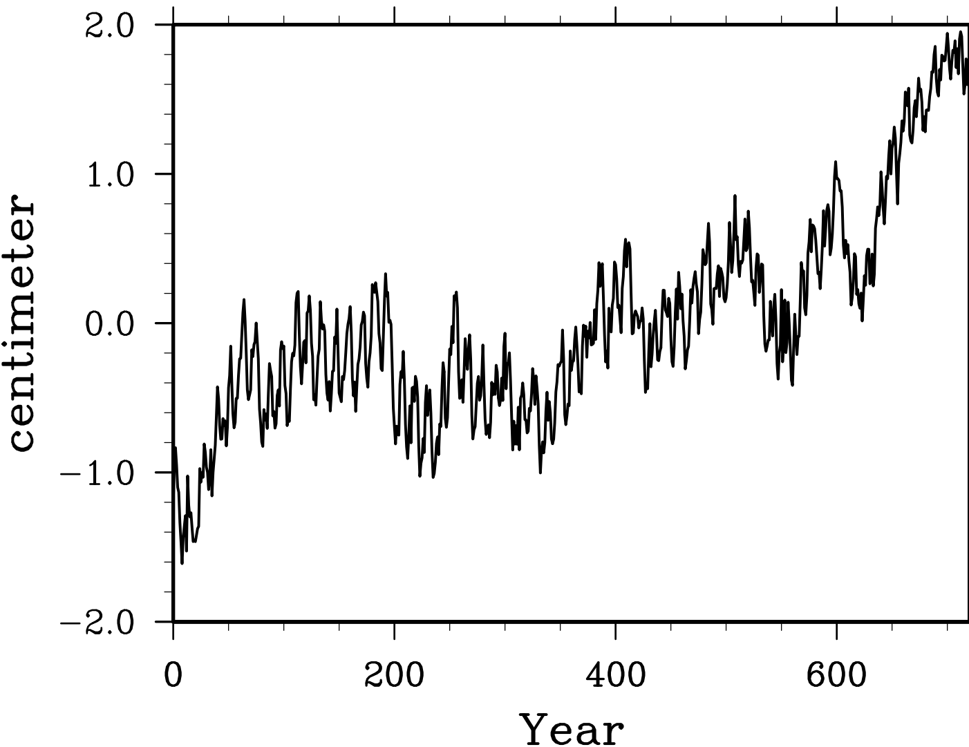
Mean Sea Level Anomaly
