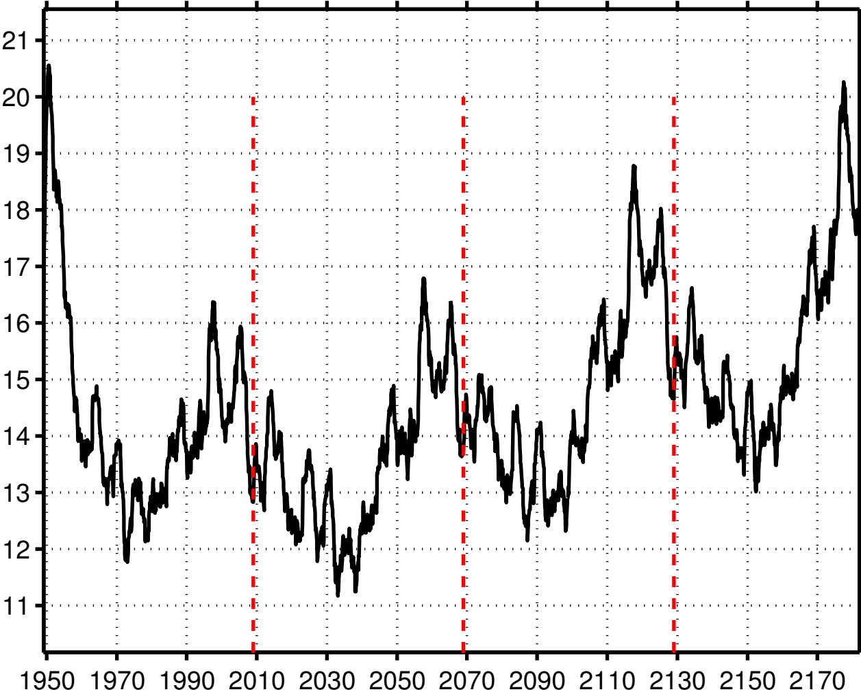
Maximum (45N) Atlantic Meridional Overturning
