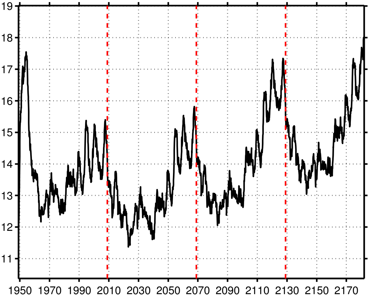
Maximum (24N) Atlantic Meridional Overturning
