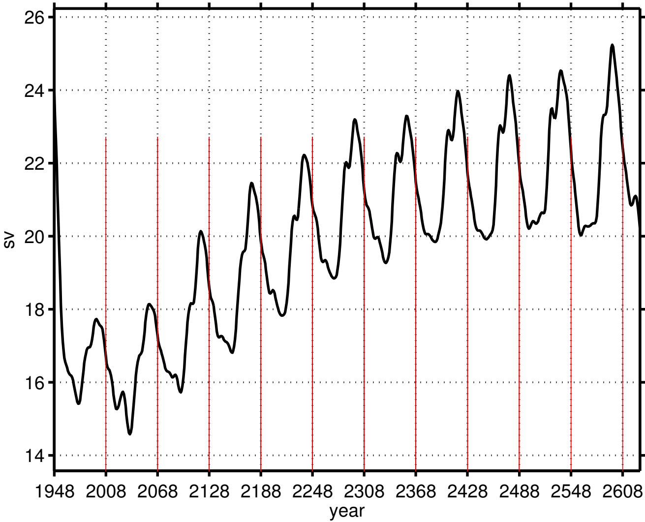
Maximum (20N–50N) Atlantic Meridional Overturning
