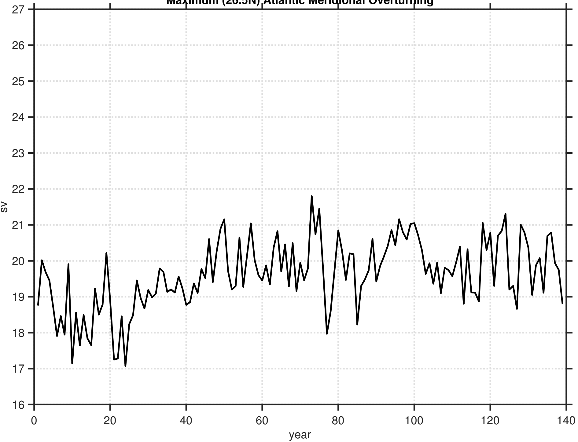
Maximum (26.5N) Atlantic Meridional Overturning
