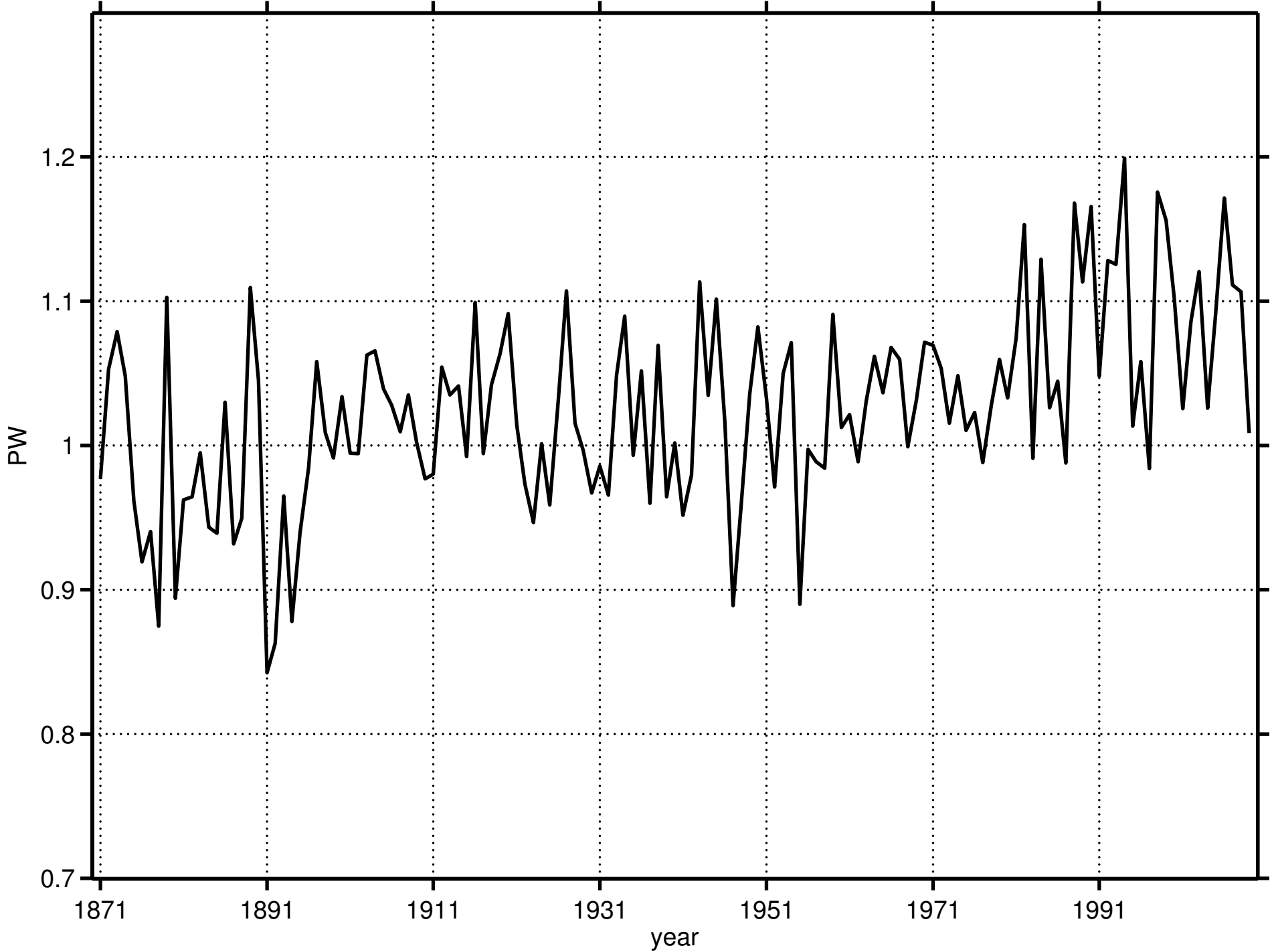
Atlantic Meridional heat transport at 26.5N
