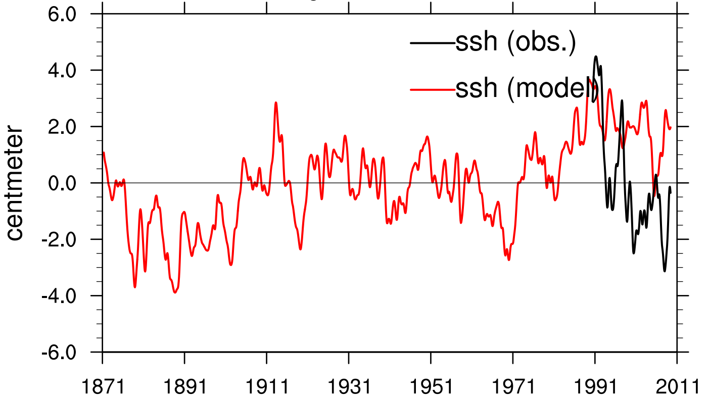
PC1 of Sea Surface Height
