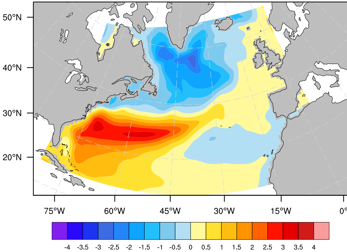
EOF1 of Sea Surface Height
