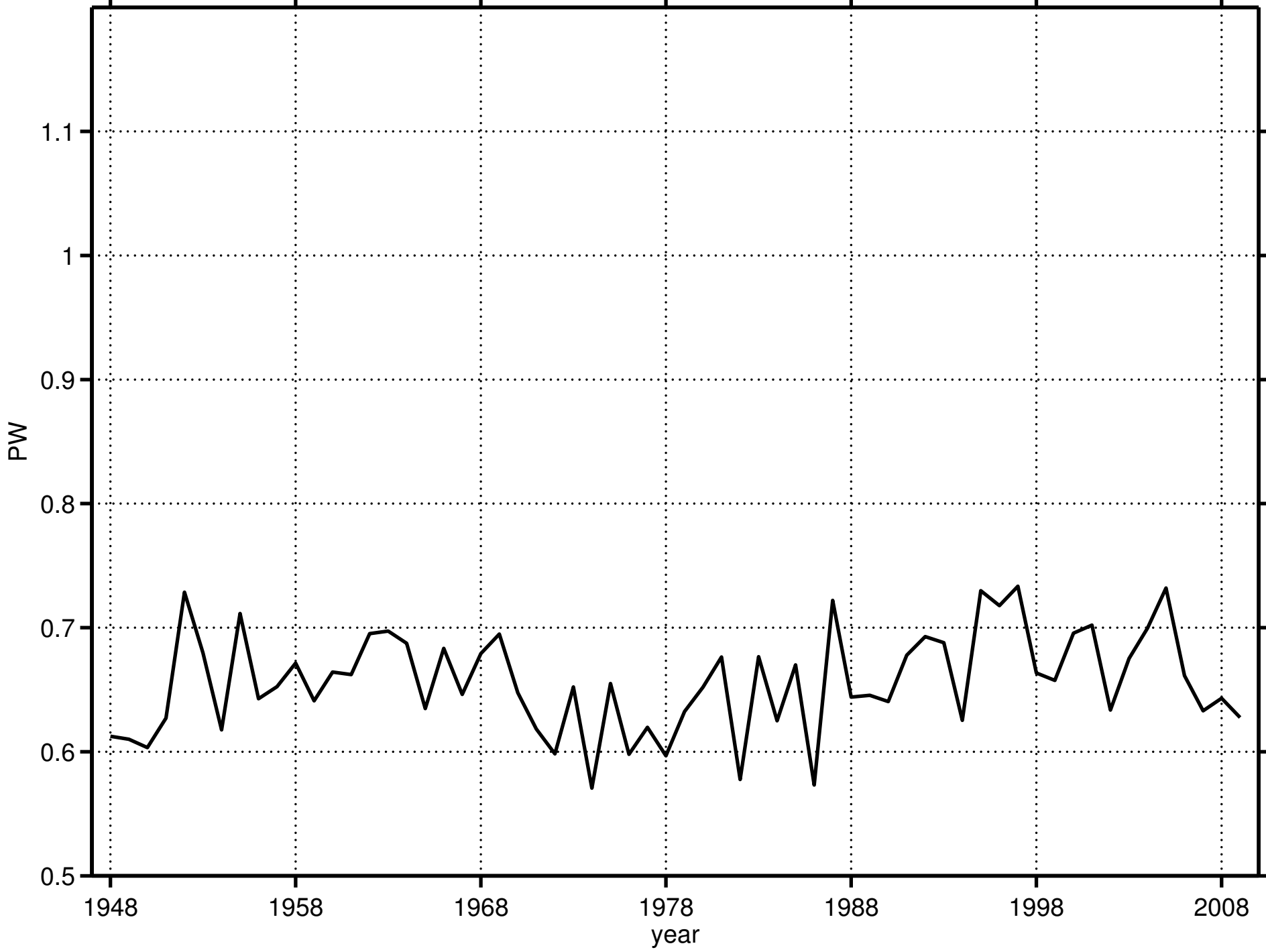
Atlantic Meridional heat transport at 47N
