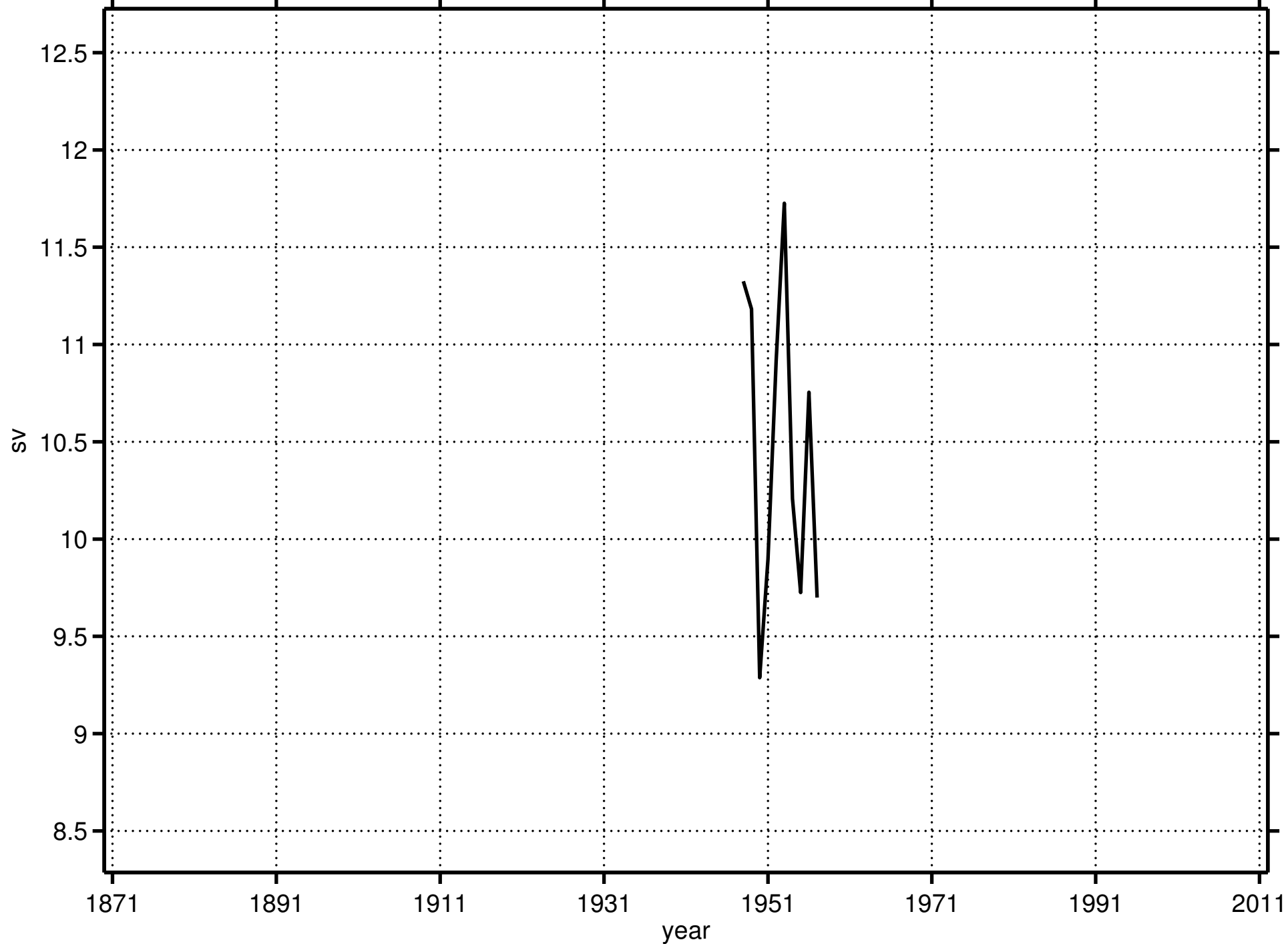
Maximum (20N–50N) Atlantic Meridional Overturning
